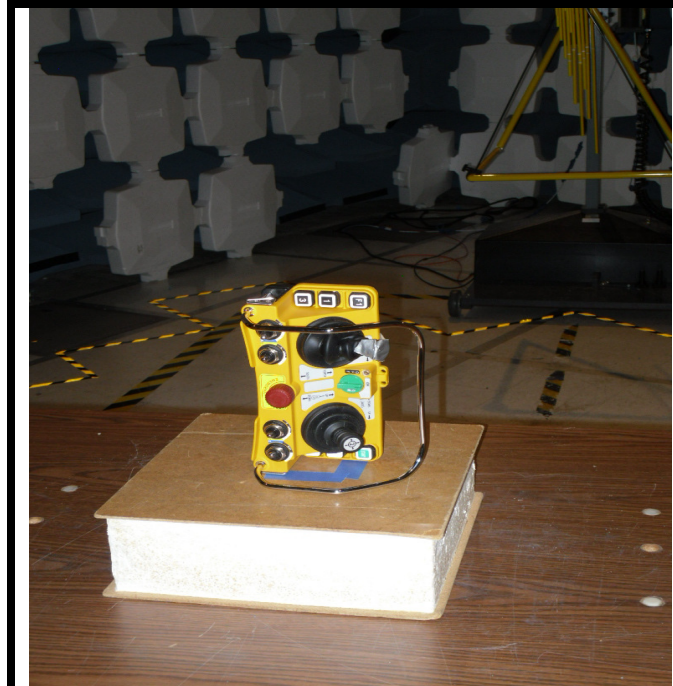
Test Setup Photo # 1
