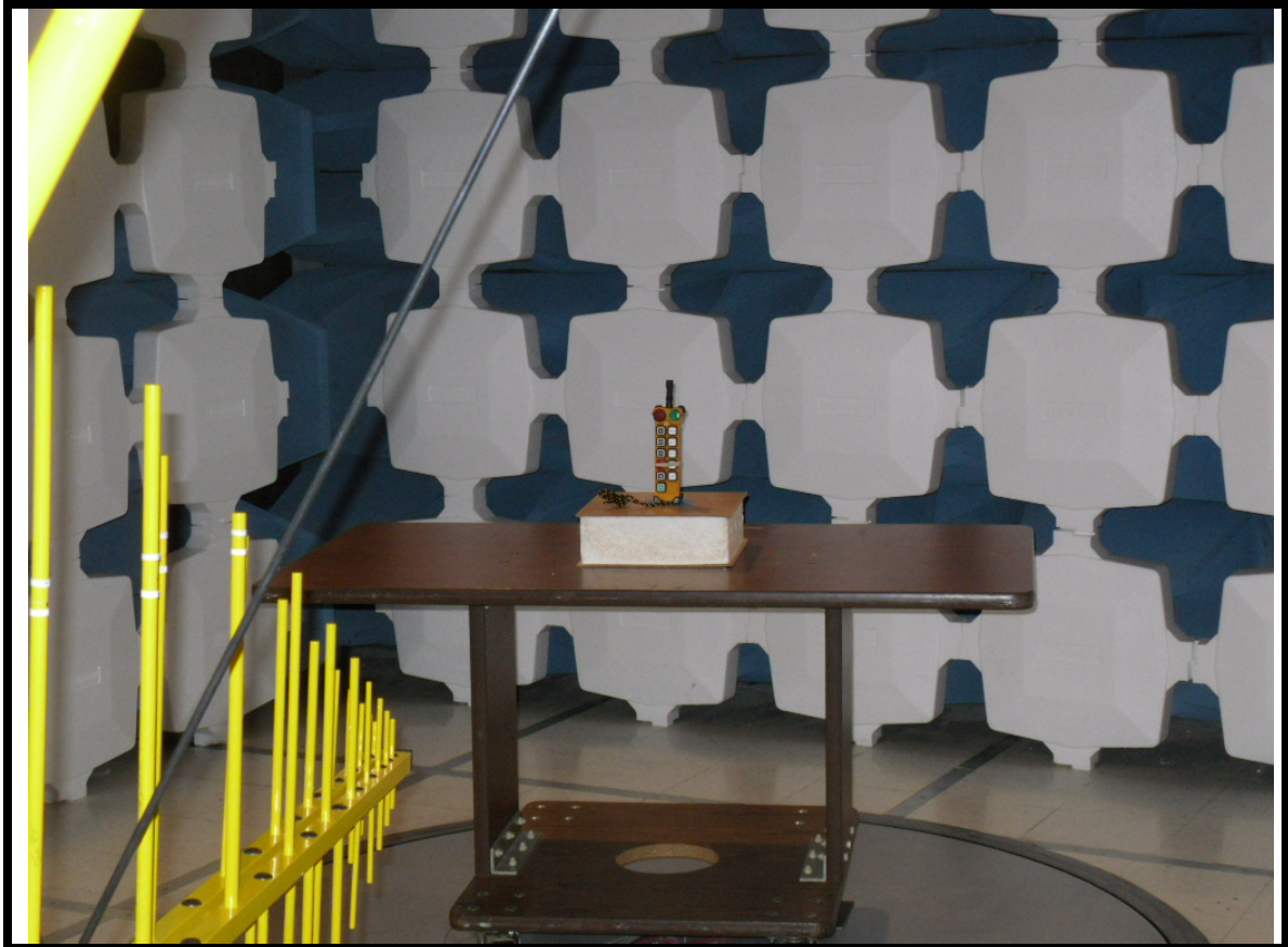
Setup Photo # 3
