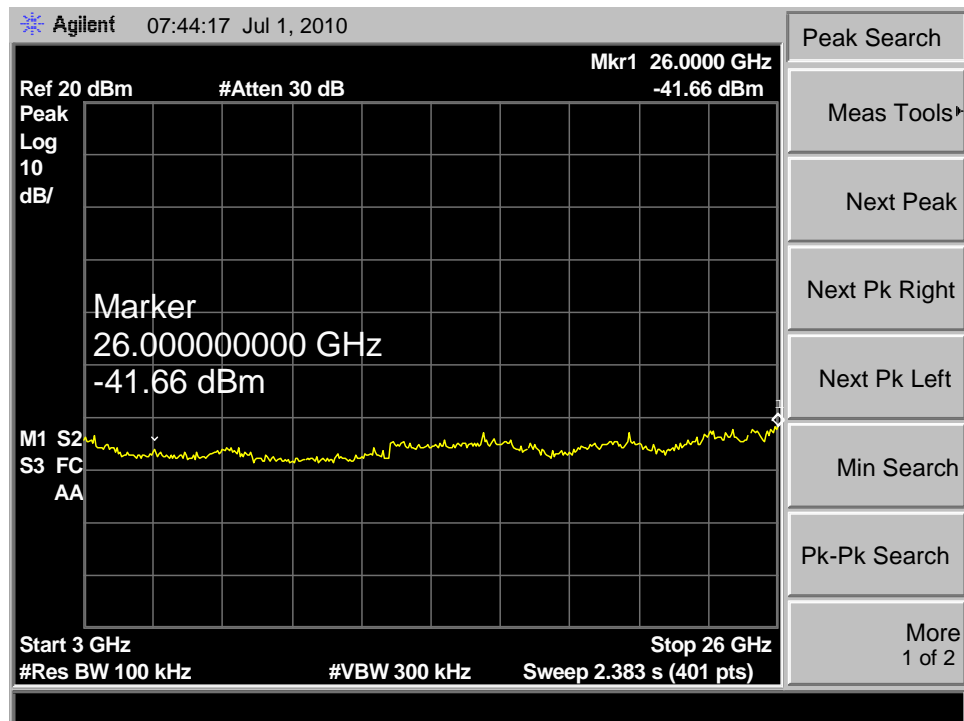
Conducted Spurious Emissions (Channel 25)
