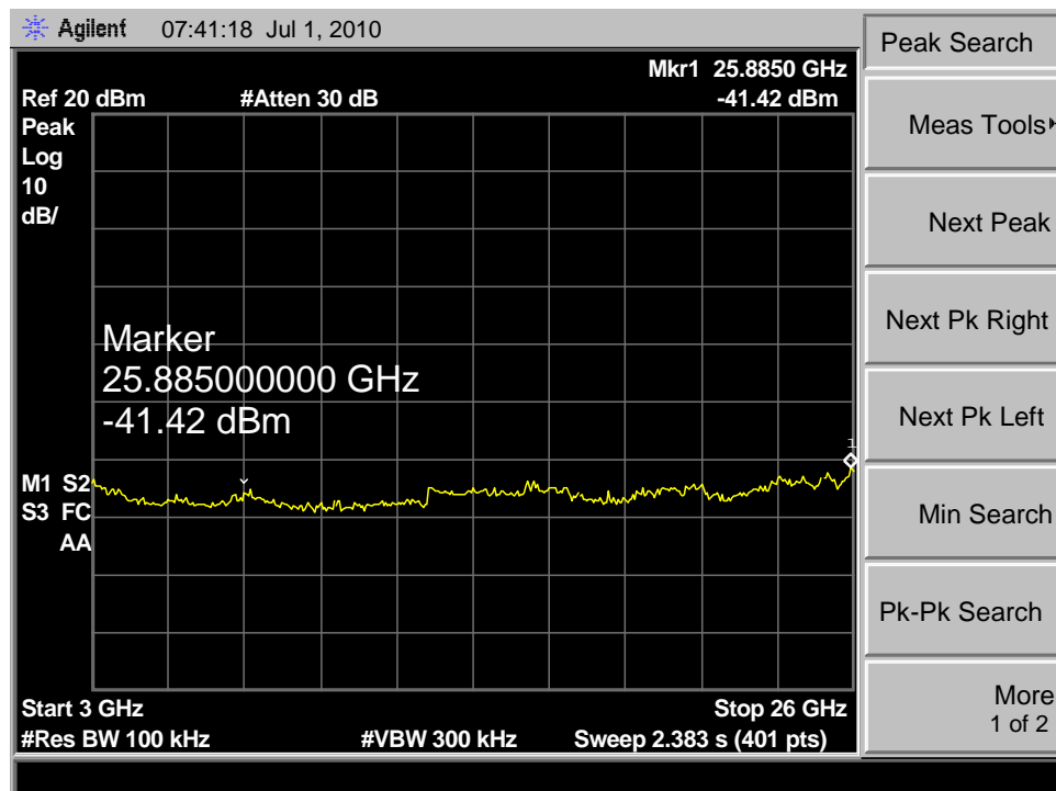
Conducted Spurious Emissions (Channel 19)
