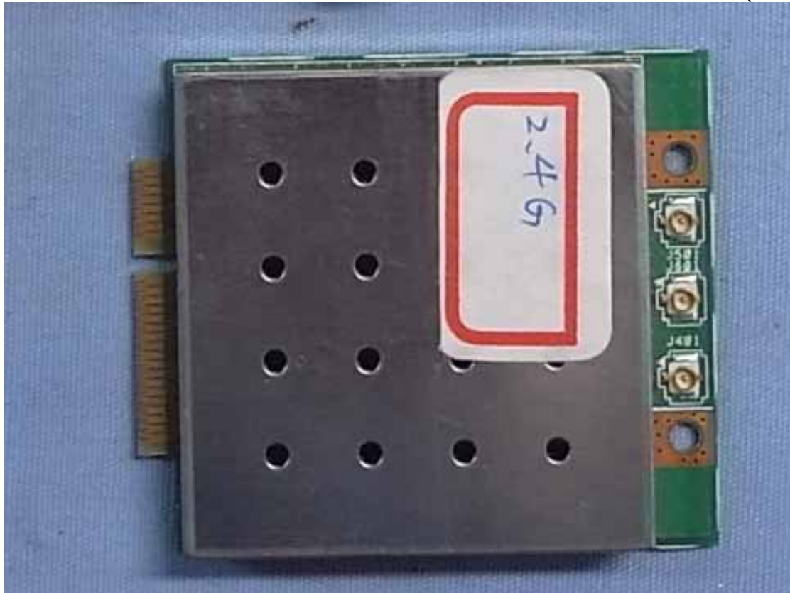
Figure 1 2.4GHz 802.11n 3T3R wifi module (Front View)
