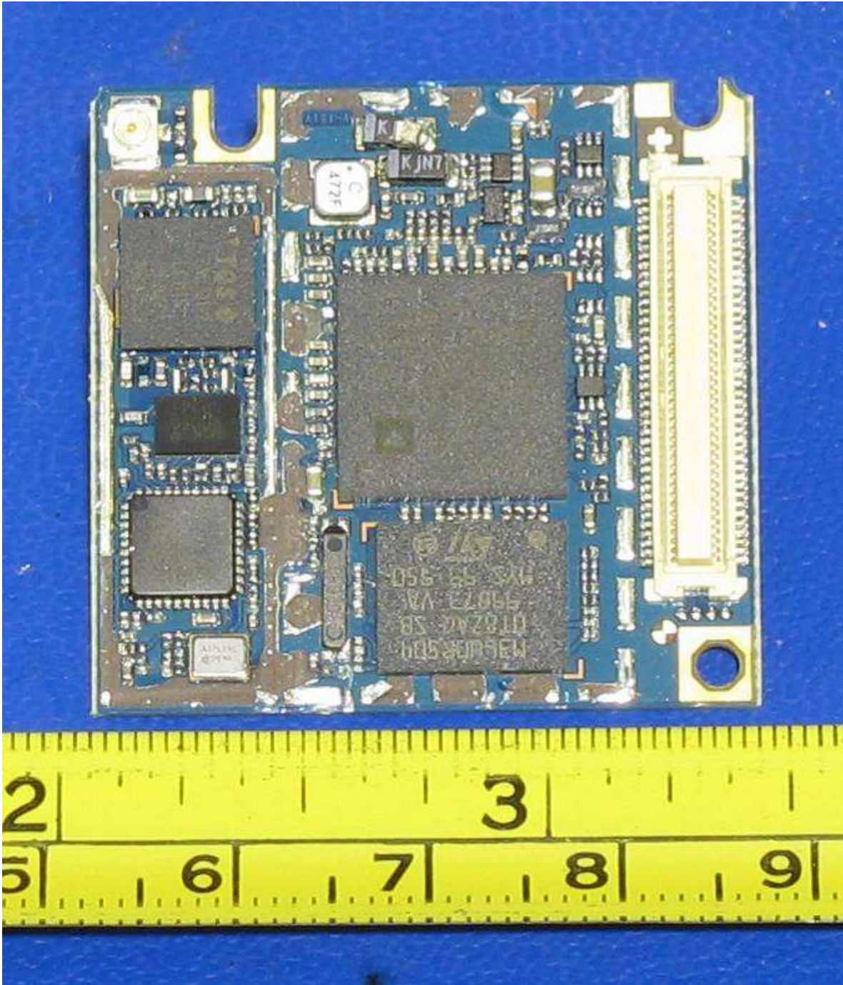
GSM Module with Shielding Removed
