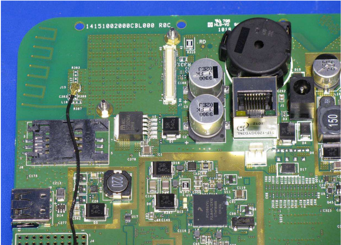
Zoomed in on GSM Module Location
