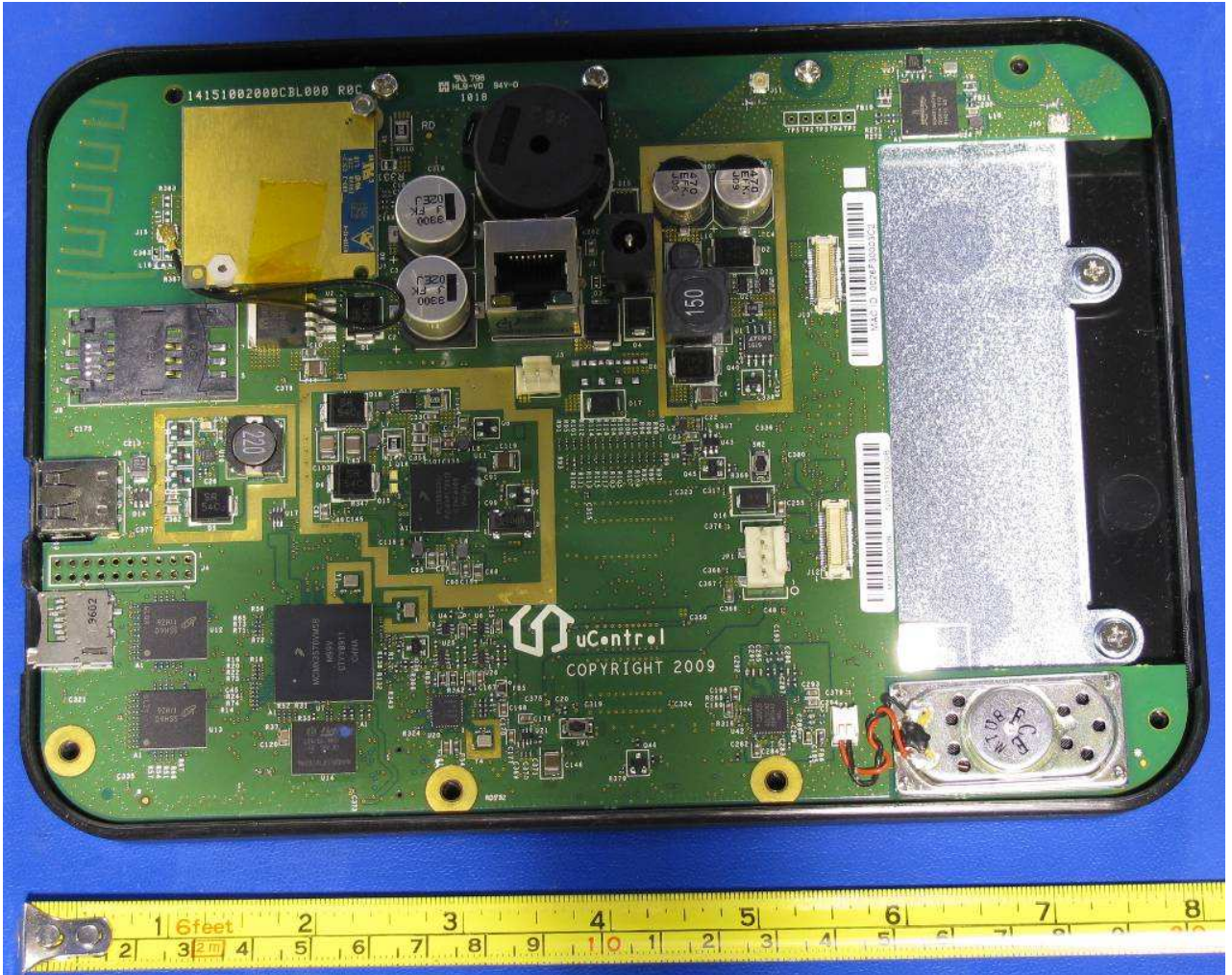
Cover Removed, Component Side of Main Board
