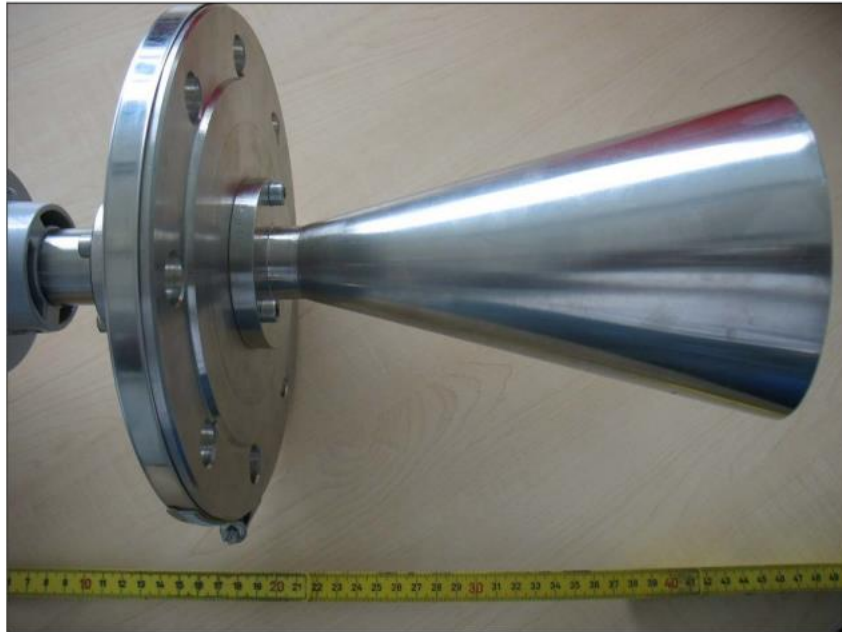
Photo 10: Metallic Horn Antenna
