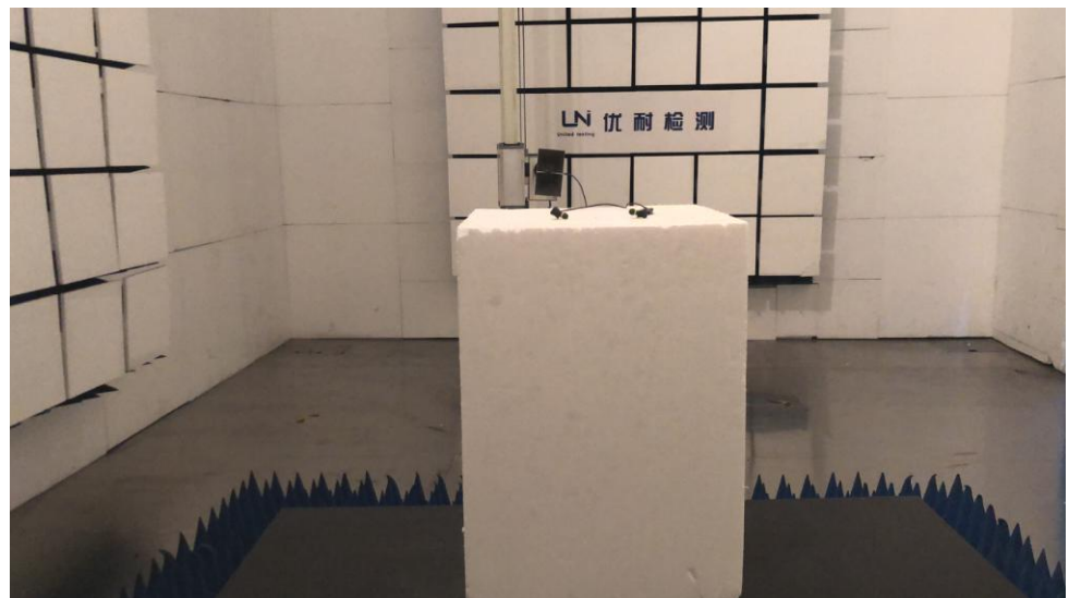
Radiated Emission (Above 1G)
