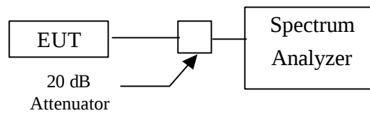
Figure 4: Emission bandwidth measurement configuration.
