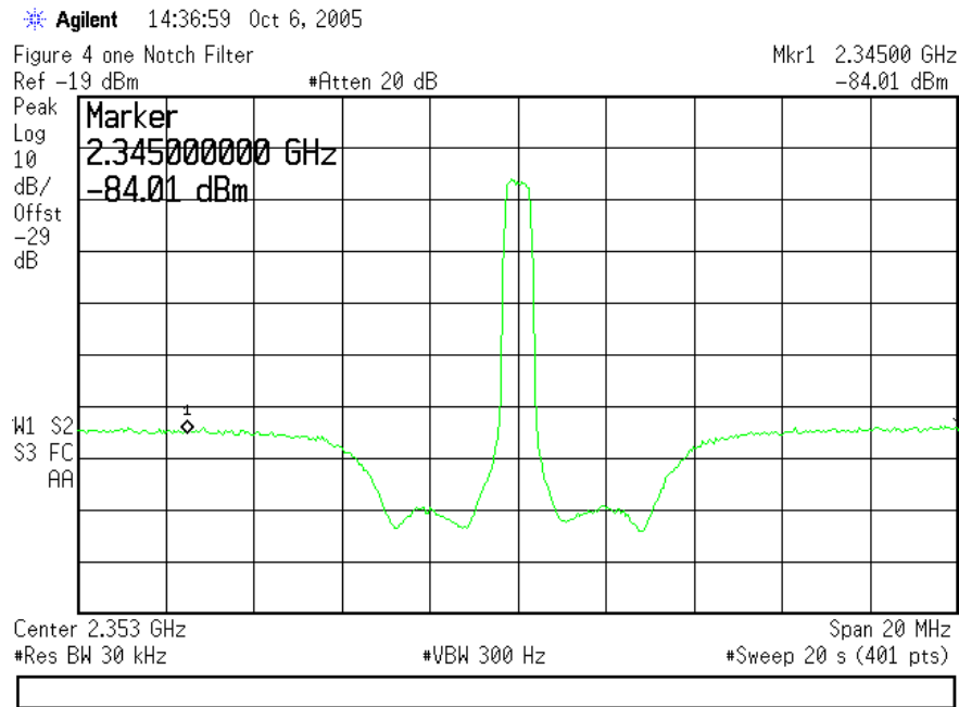
FIGURE 4. Typical Notch Filter
