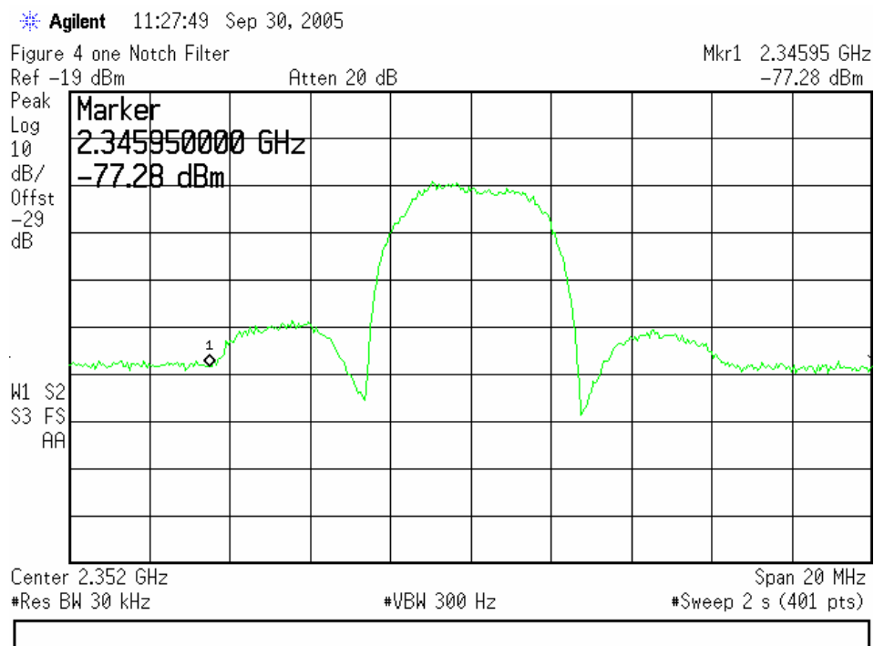
FIGURE 4. Typical Notch Filter
