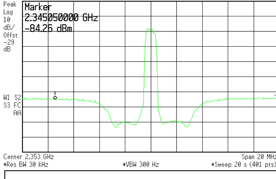
FIGURE 4. Typical Notch Filter
