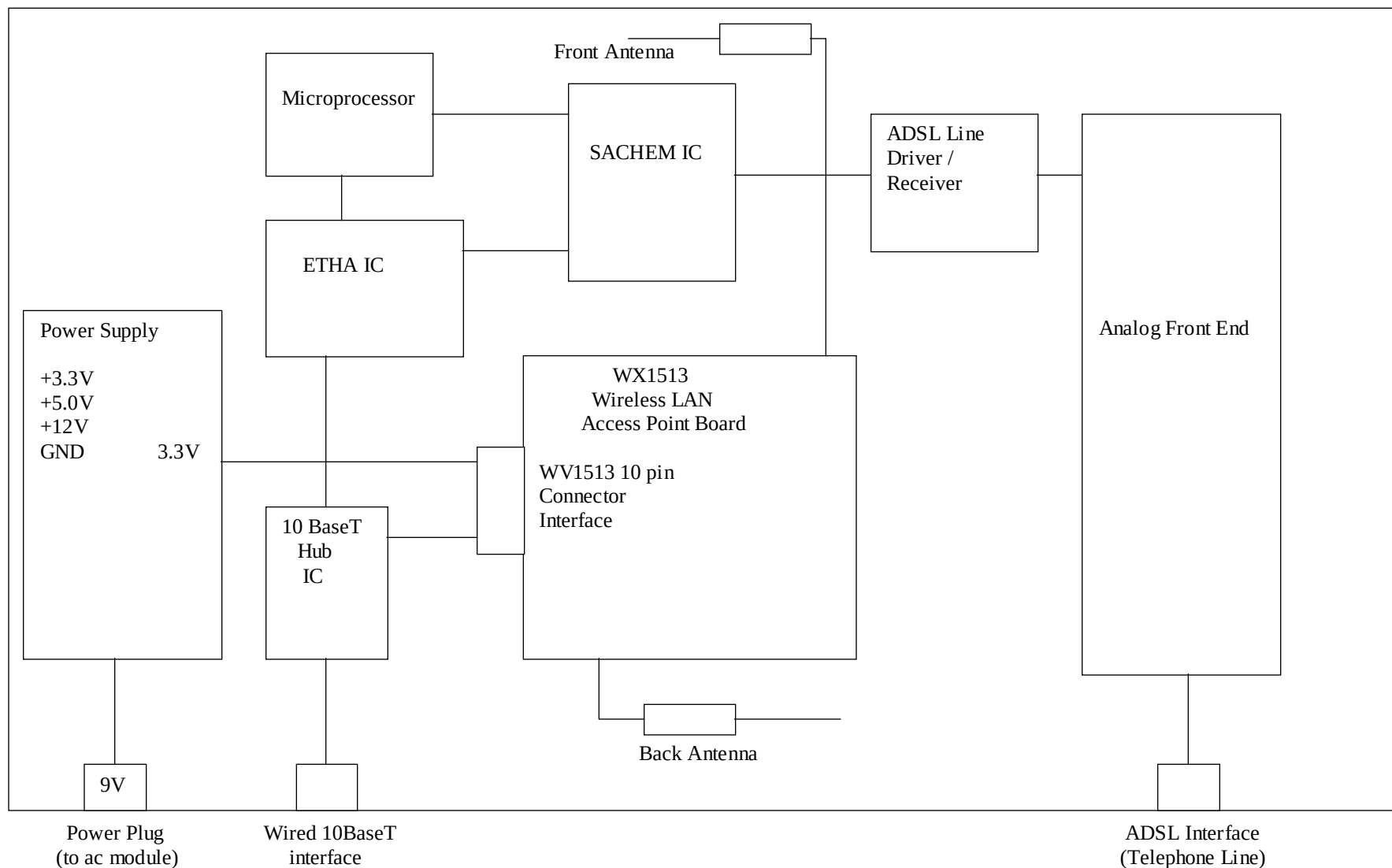
BLOCK DIAGRAM, 3EC18883 ADSL WIRELESS MODEM
