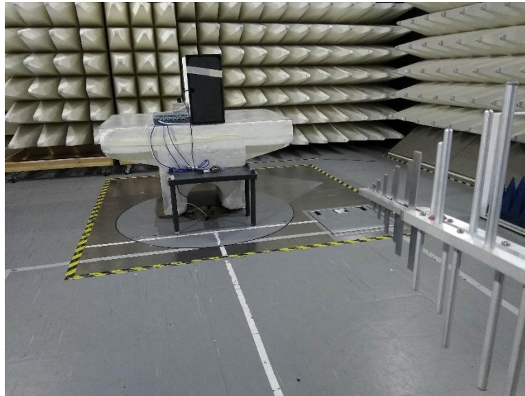
Photograph No.2 Setup for carrier field strength measurements in the anechoic chamber in 30 – 1000 MHz range
