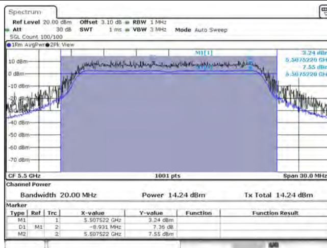
5470-5725MHz - Worst RF Output Power Plots
