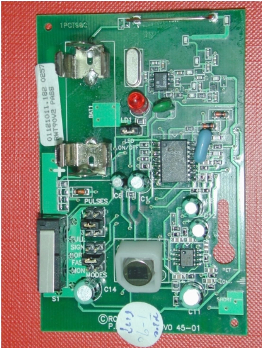
Photograph No.1 RWT90V2 detector PCB front view
