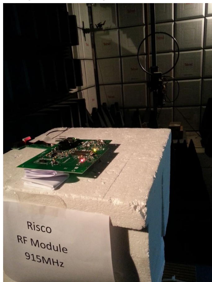
Figure 3. Radiated Emission Test
