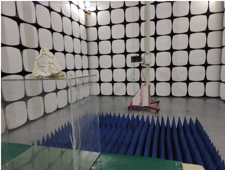
Radiated Emission test view (Frequency from 1GHz to 18GHz)
