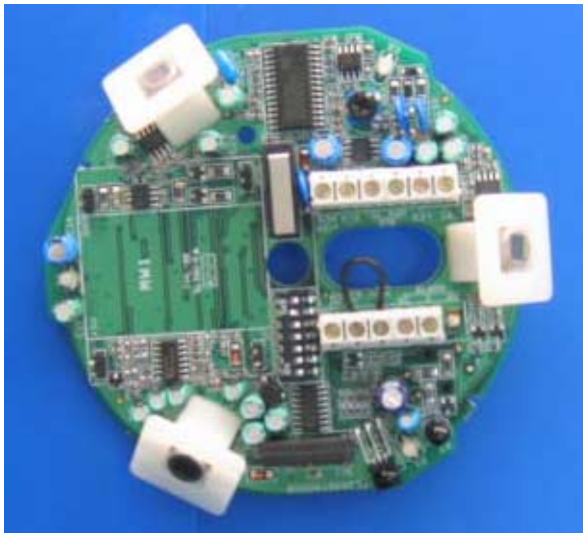
Photograph No.4 Component side of the main PCB with the Tx board removed
