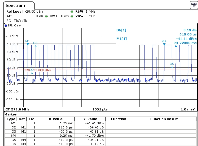
Figure 5: Fundamental Emission Pulsed Operation.
