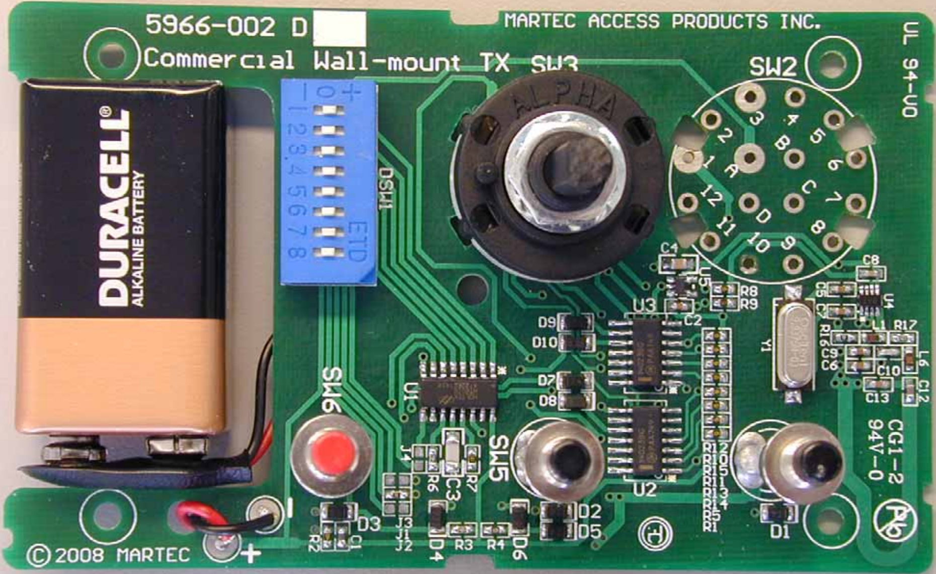
PCB (top)
