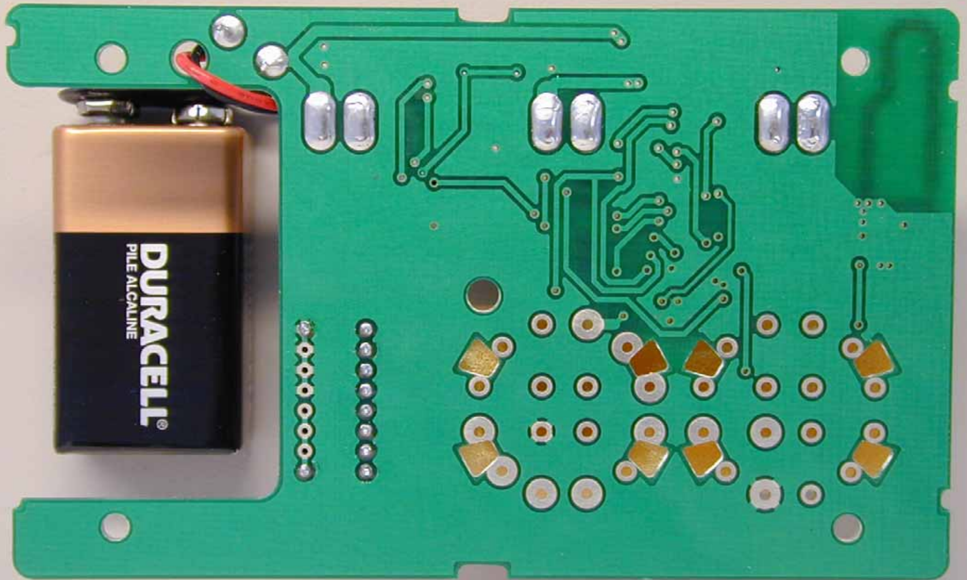
PCB (bottom)
