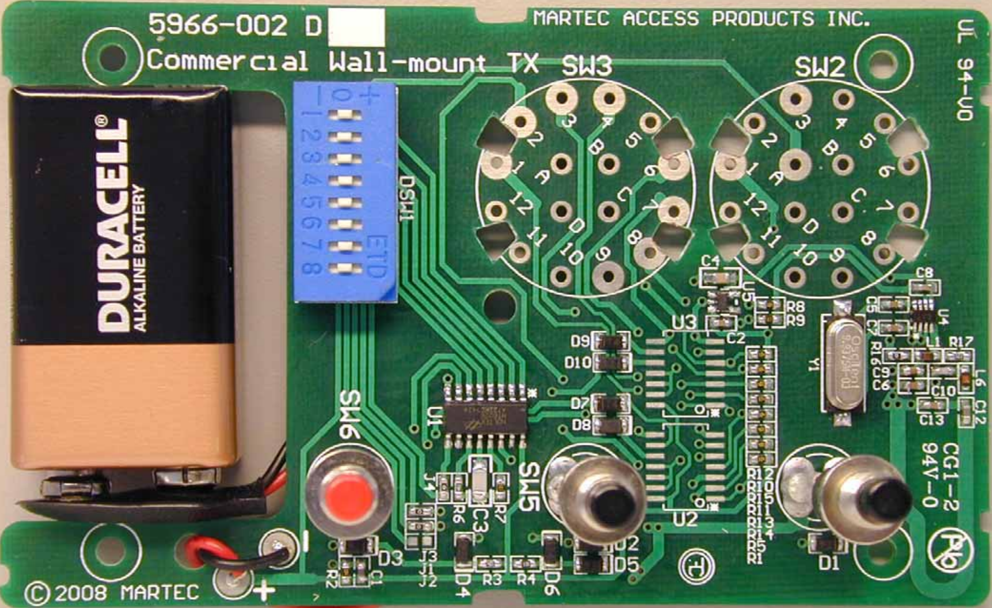
PCB (top)
