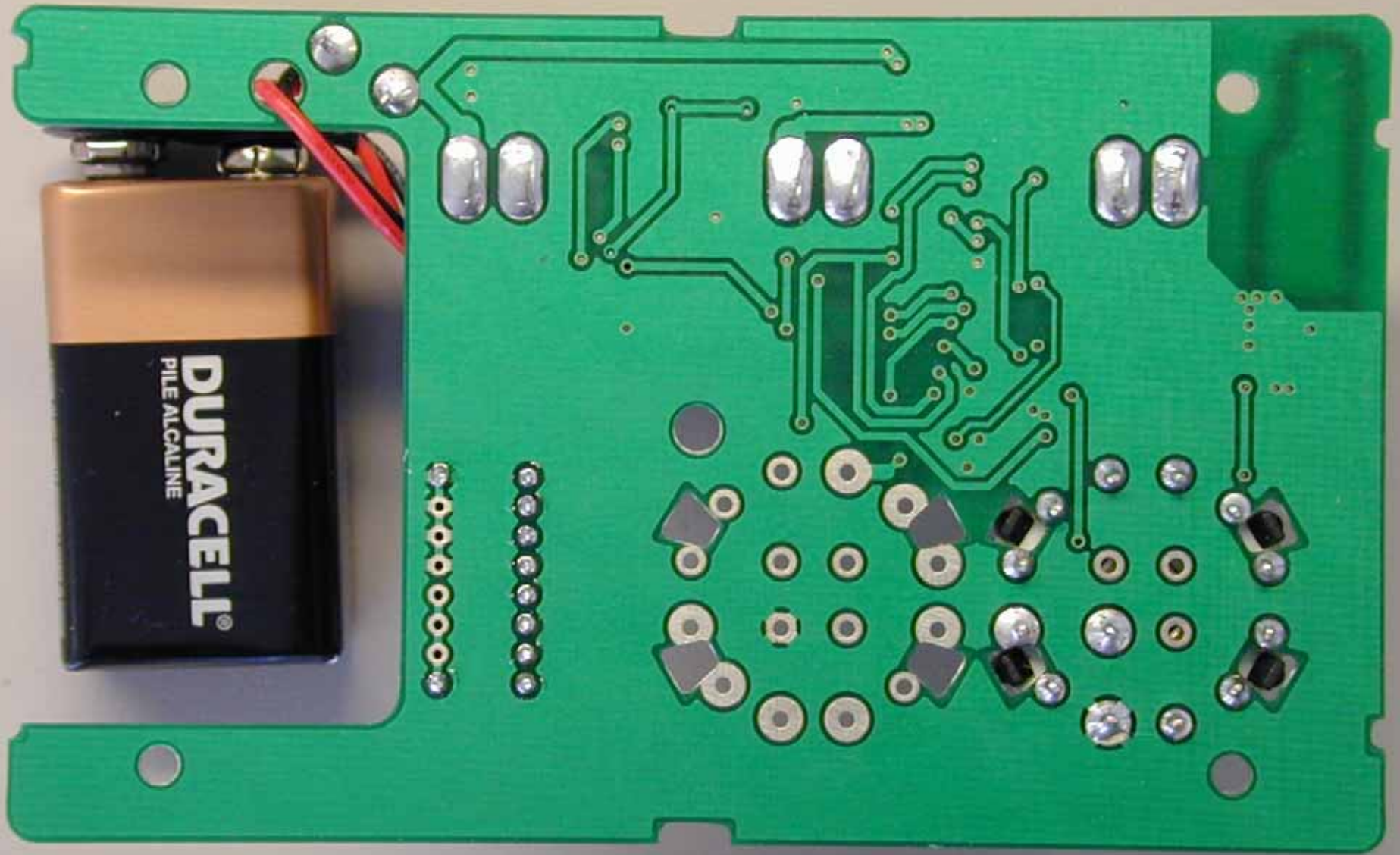
PCB (bottom)
