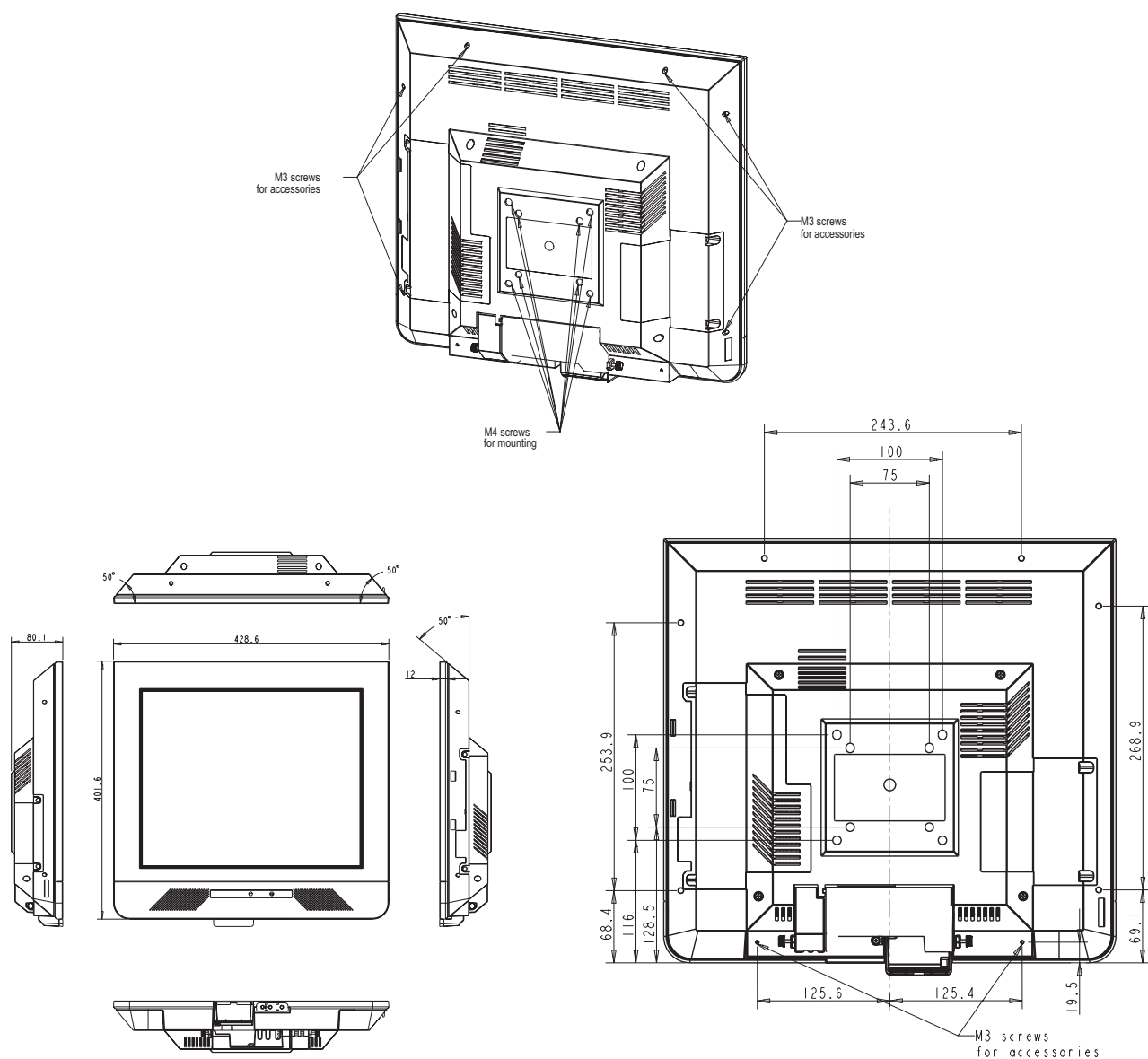
Figure 35. Dimensions for 17 inch models
