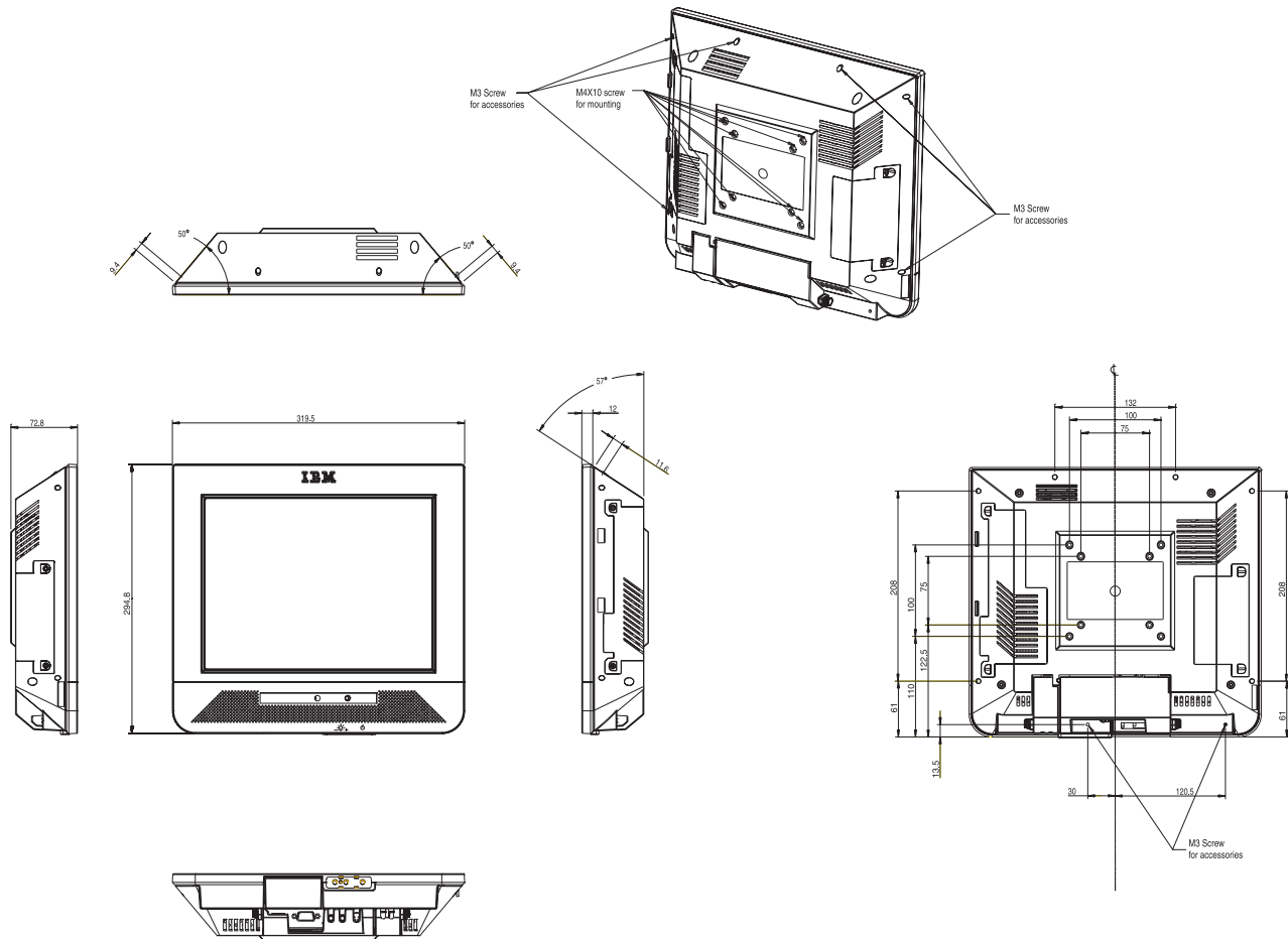
Figure 33. Dimensions for 12 inch models
