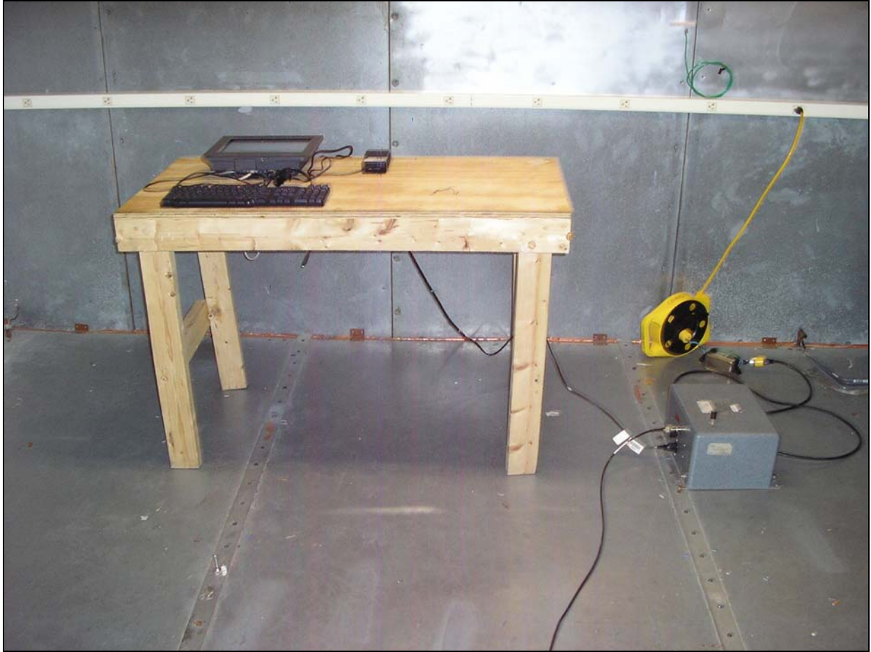
Photograph 1. Conducted Emissions, 12" Model, Test Setup
