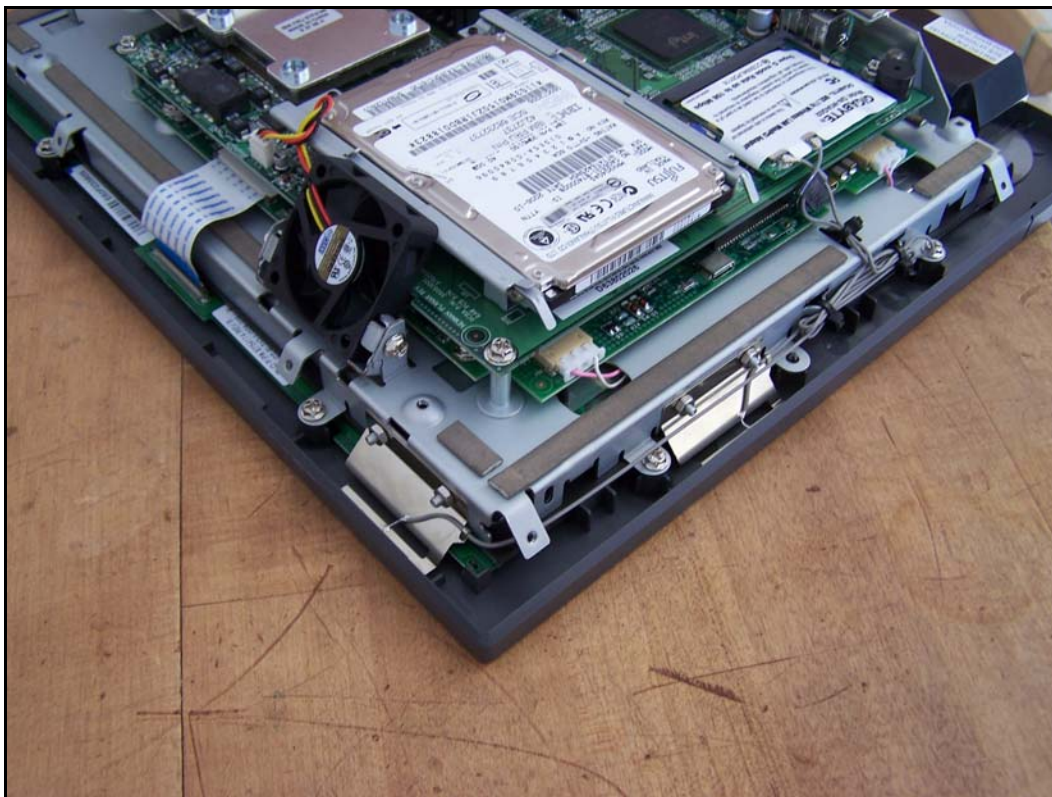
Photograph 4. Internal Photo of 12" Model
