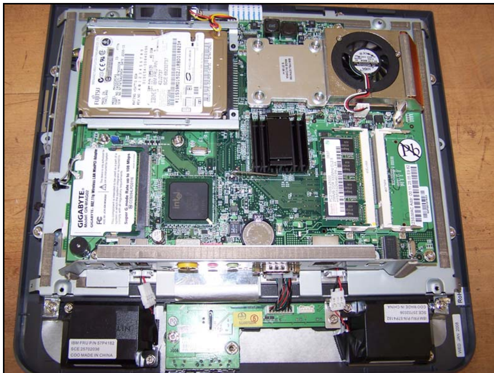
Photograph 2. Internal Photo of 12" Model
