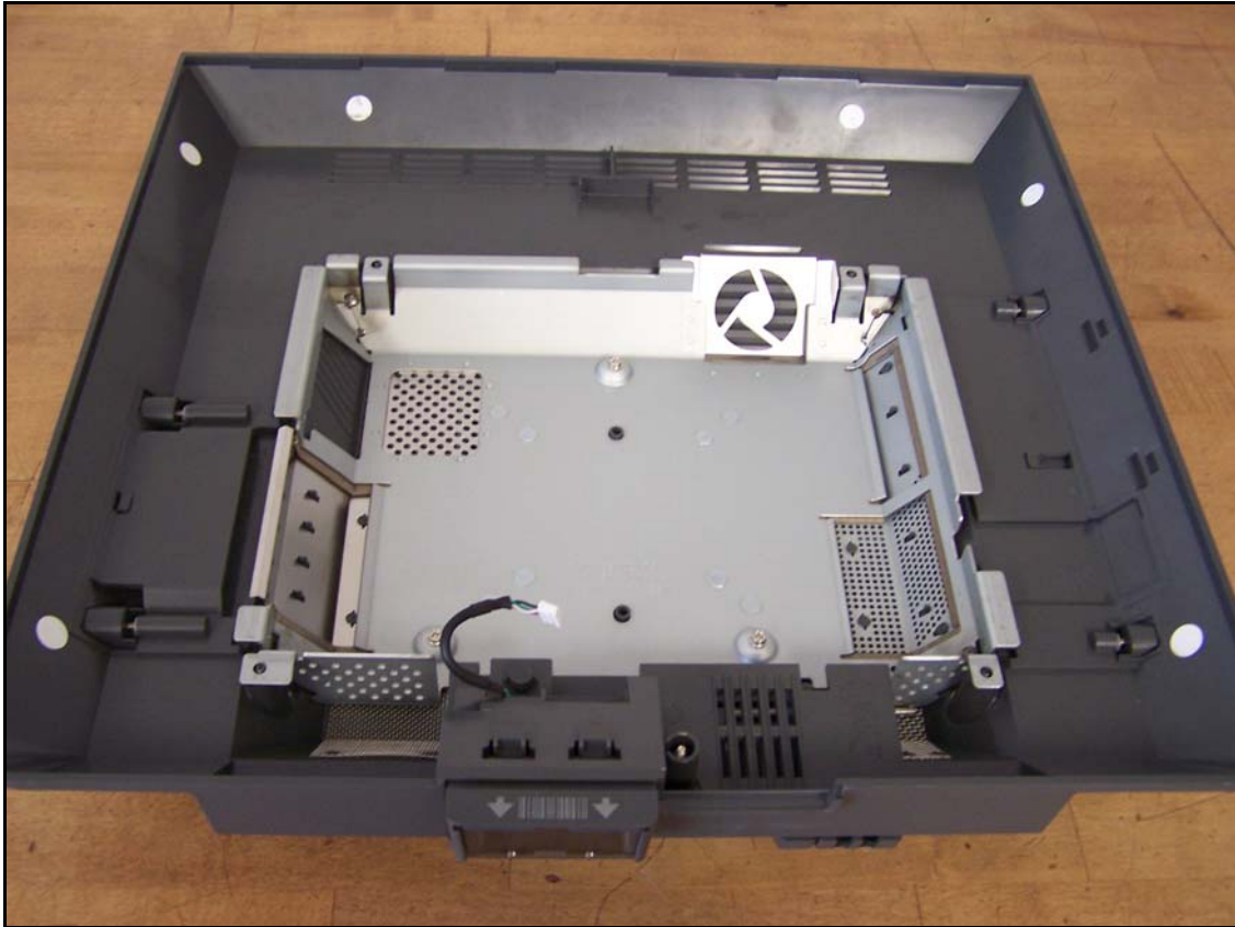
Photograph 11. Internal Photo of 17'' Model
