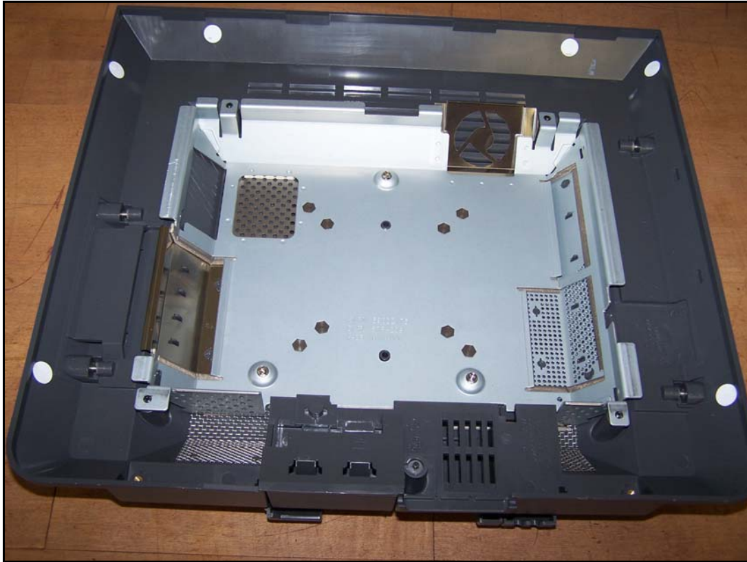
Photograph 6. Internal Photo of 15'' Model
