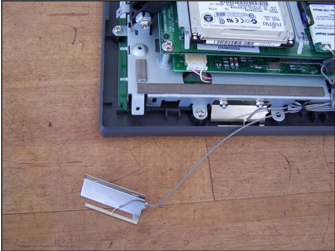
Photograph 5. Internal Photo of 12" Model
