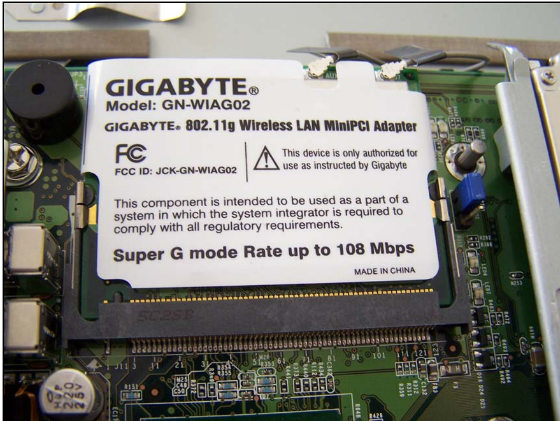
Photograph 8. Internal Photo of 15" Model
