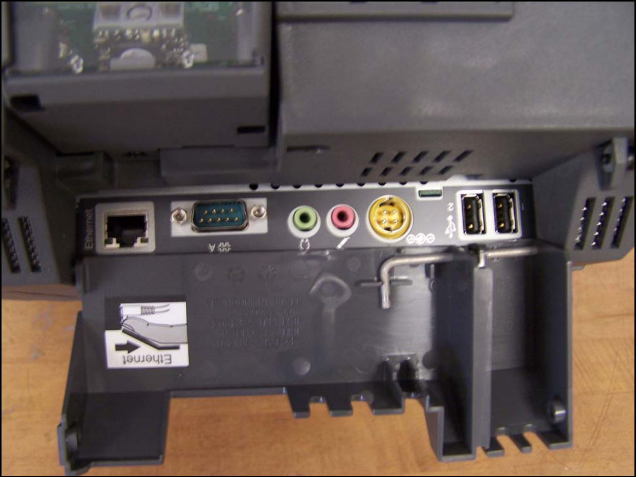
Photograph 9. External Photo of Bottom Connector Panel of the 17" Model
