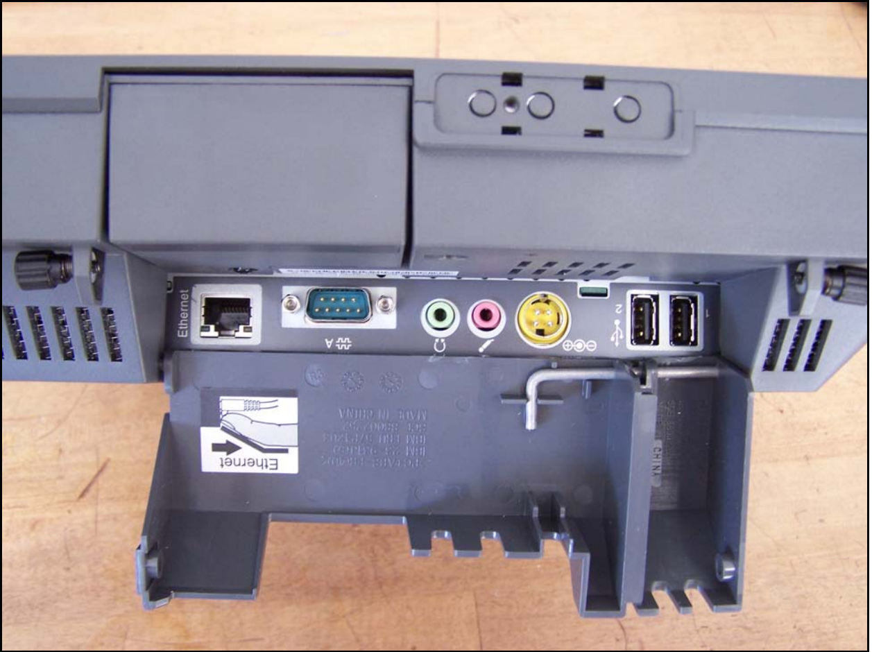
Photograph 3. External Photo of Bottom Connector Panel of the 12" Model
