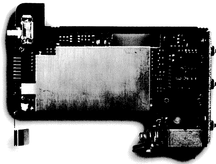
MODEL CP-AV03 HH BAND LOGIC BOARD SIDE 1
