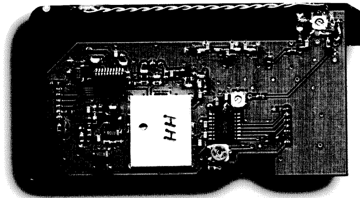
MODEL CP-AV03 HH BAND RX SIDE2
