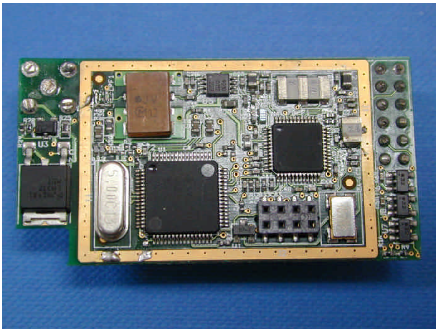
Transceiver module without shield, first side
