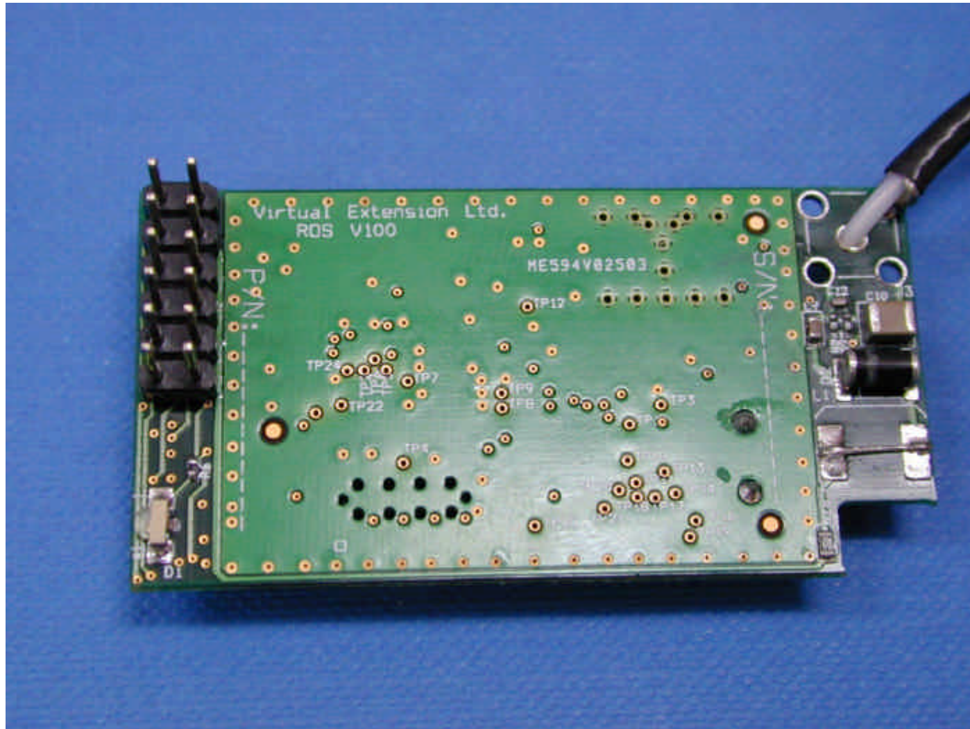
Transceiver module, second side
