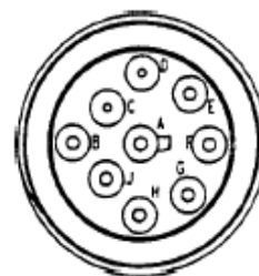
View into 1708CAB9 Connector
