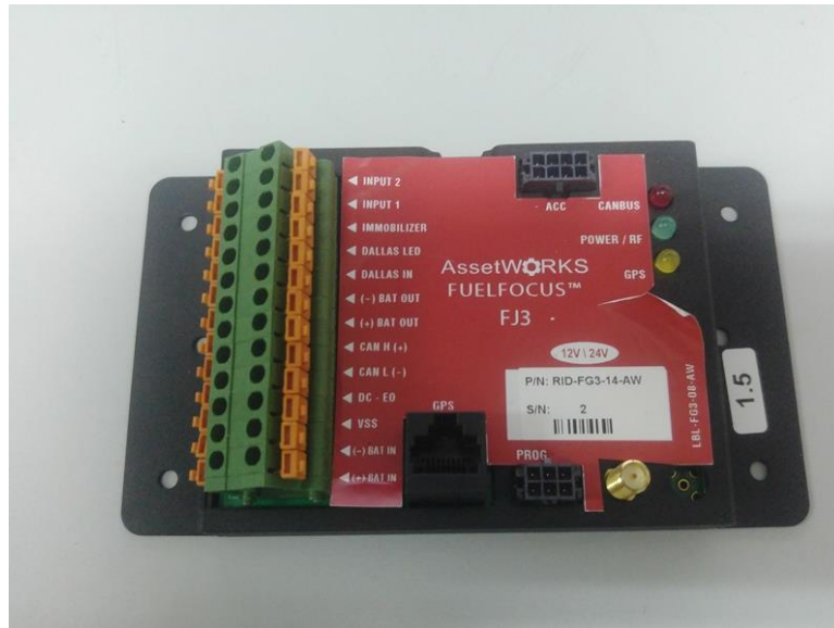
Photograph No.2 Car Data Logger without SMA connector general view
