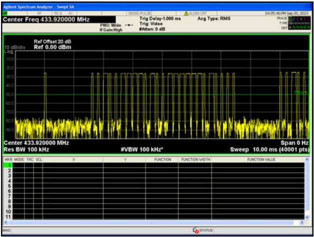
Period-10ms
