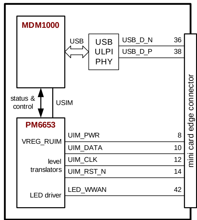
Figure 5-1 UNDP-1 communication interfaces
