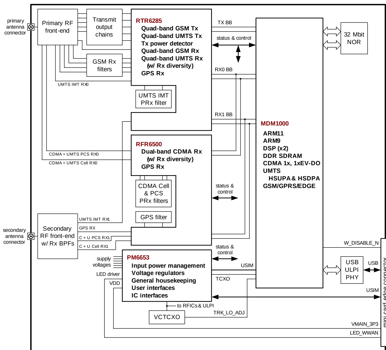
Figure 1-2 Example application functional block diagram
