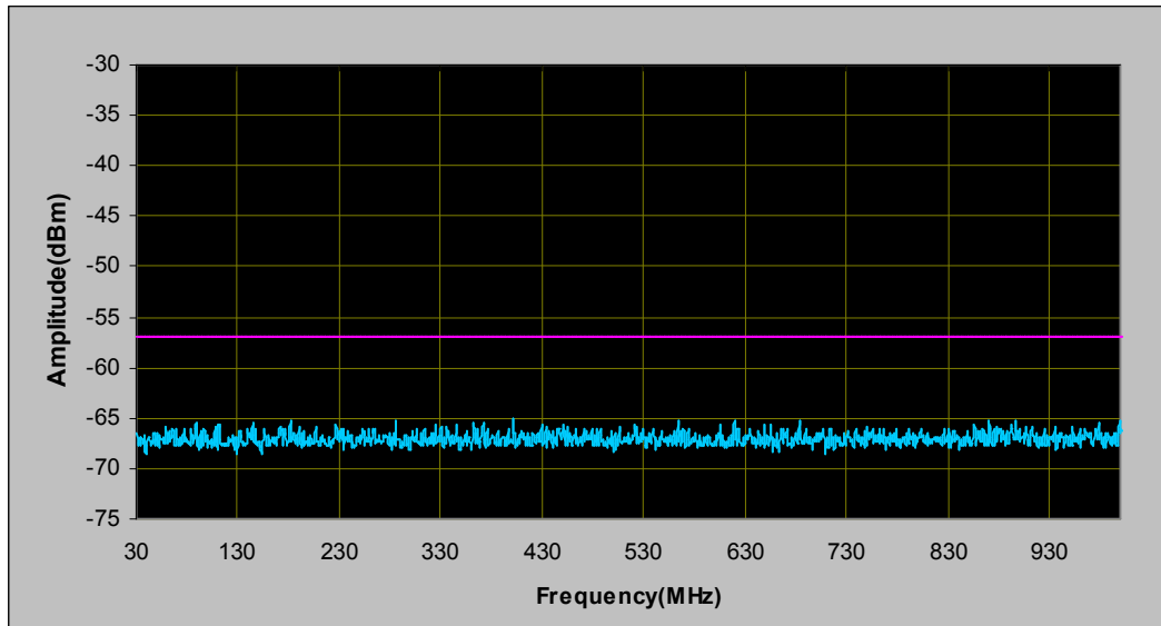
Receiver Spurious Emission (WCDMA Band II, channel 9400) Plot- 1
