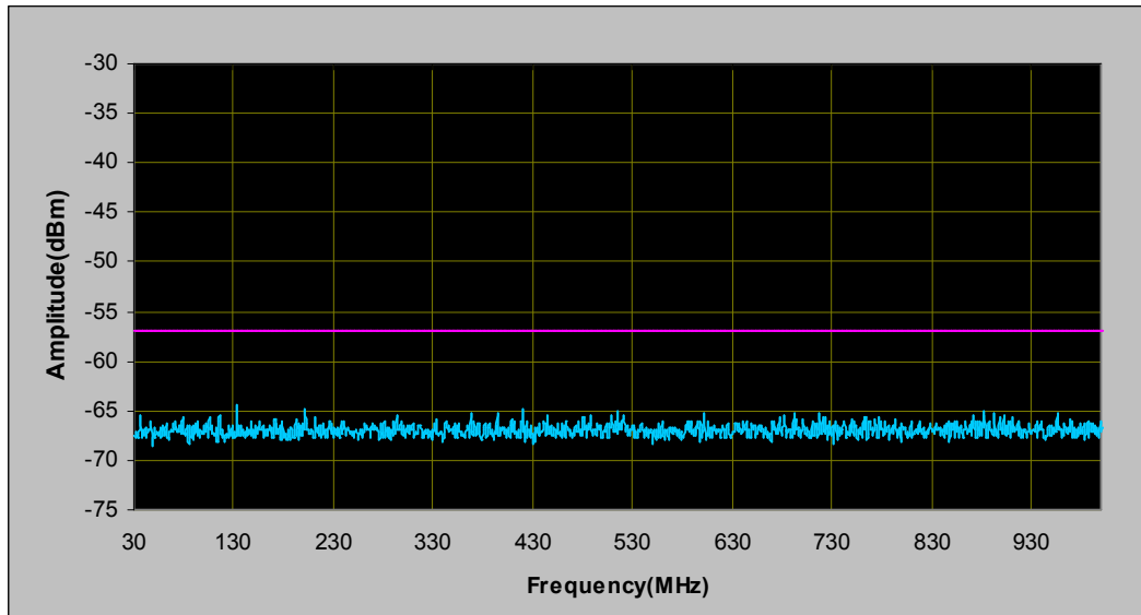
Receiver Spurious Emission (GSM / GPRS850, channel 189) Plot- 1
