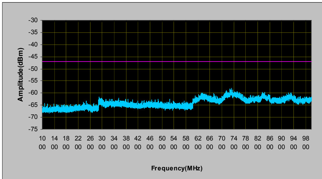
Receiver Spurious Emission (GPRS850, channel 189) Plot- 2
