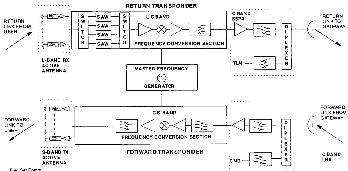
Figure 2-13 Communications Payload Simplified Block
