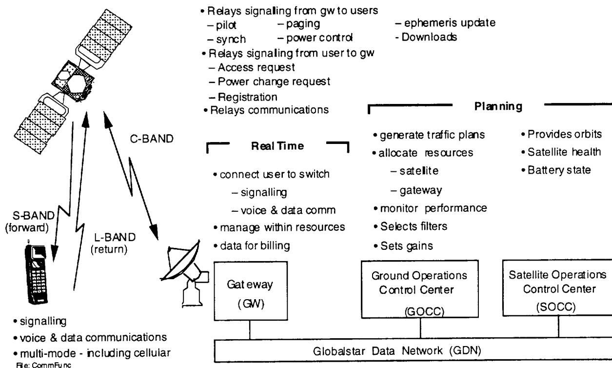
Figure 2-9 Ground Segment Support for Communications
