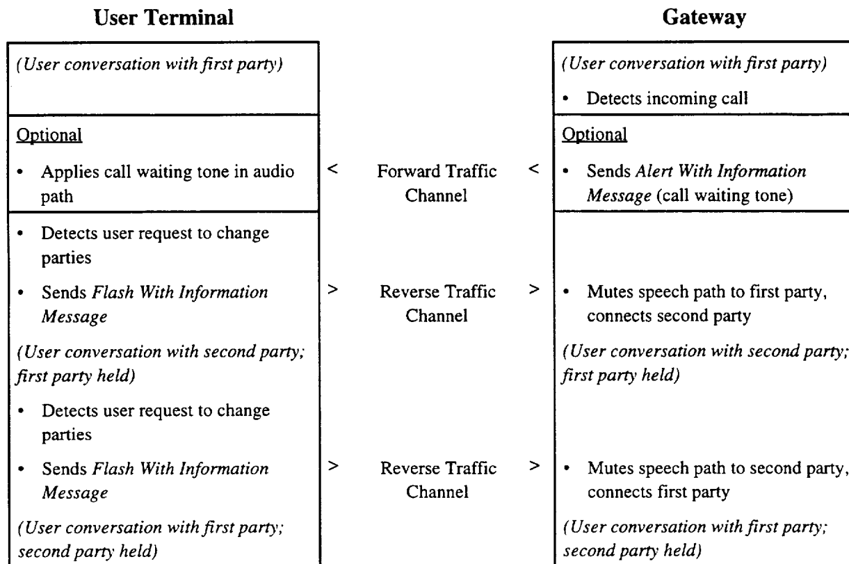
Figure 6-13. Simple Call Flow, Call-Waiting Example (TIA Call Control Procedures)
