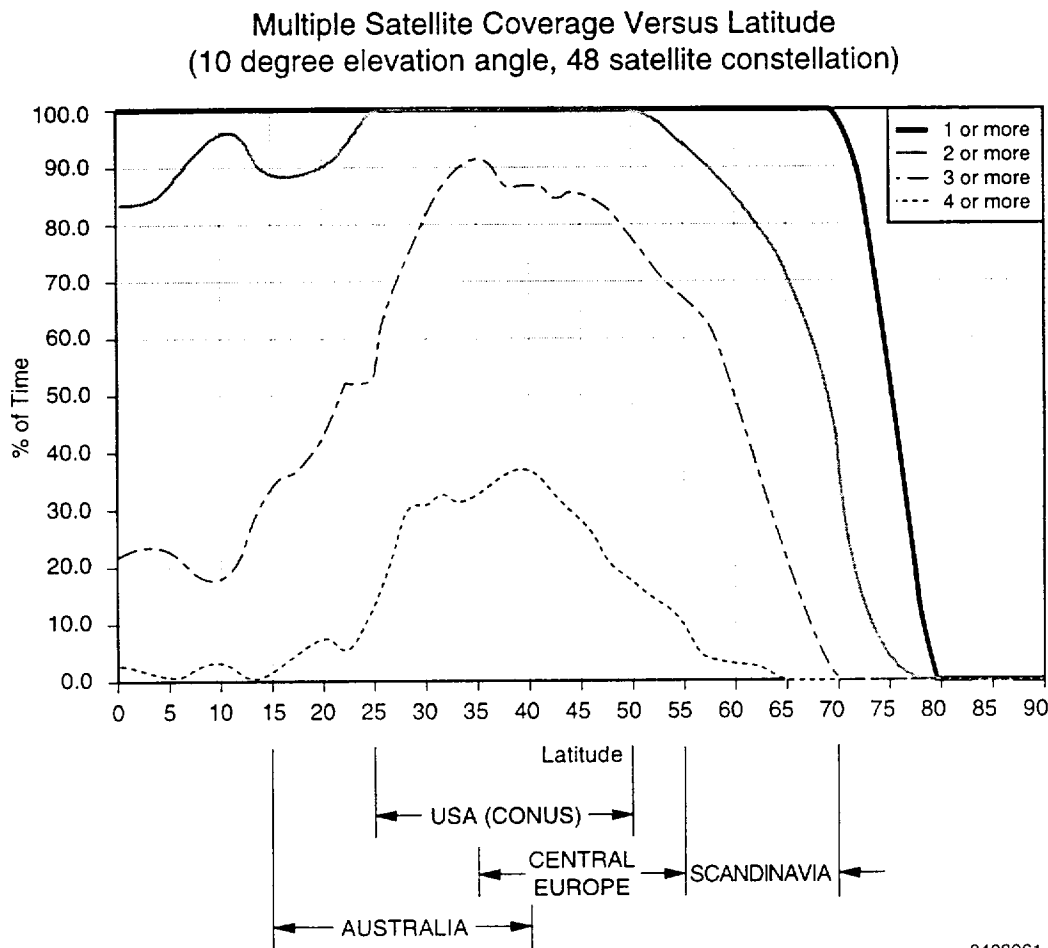
Figure 3-7 Enhanced Coverage for Temperate Regions
