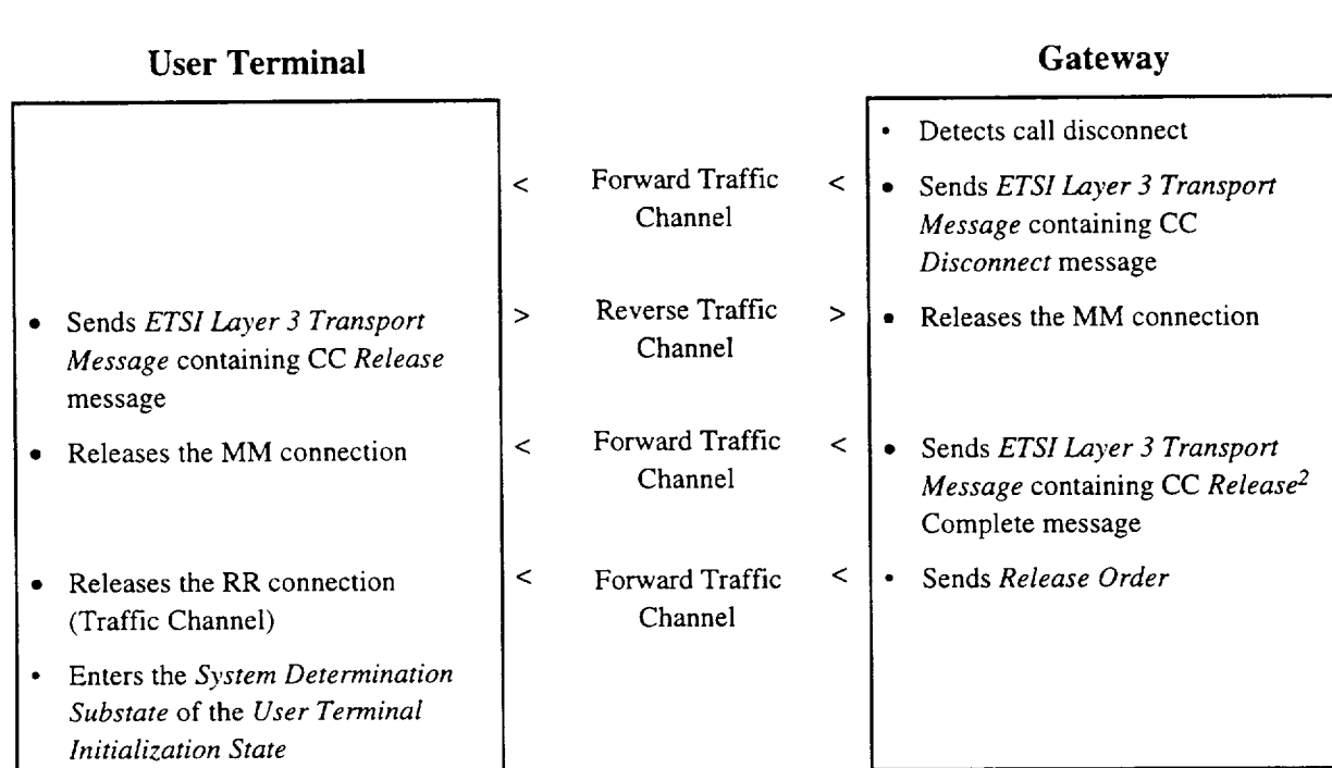
3 Figure 6-11 Simple Call Flow, Gateway Initiated Call Disconnect Example (ETSI Call 4 Control Procedure) 5 (Part 2 of 2) 6
