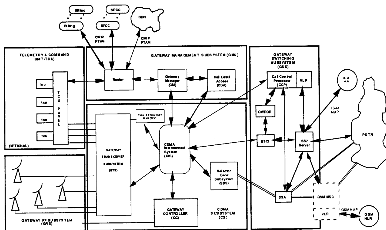
Figure 5-2 Gateway Connections to the PSTN - Flexible Interface
