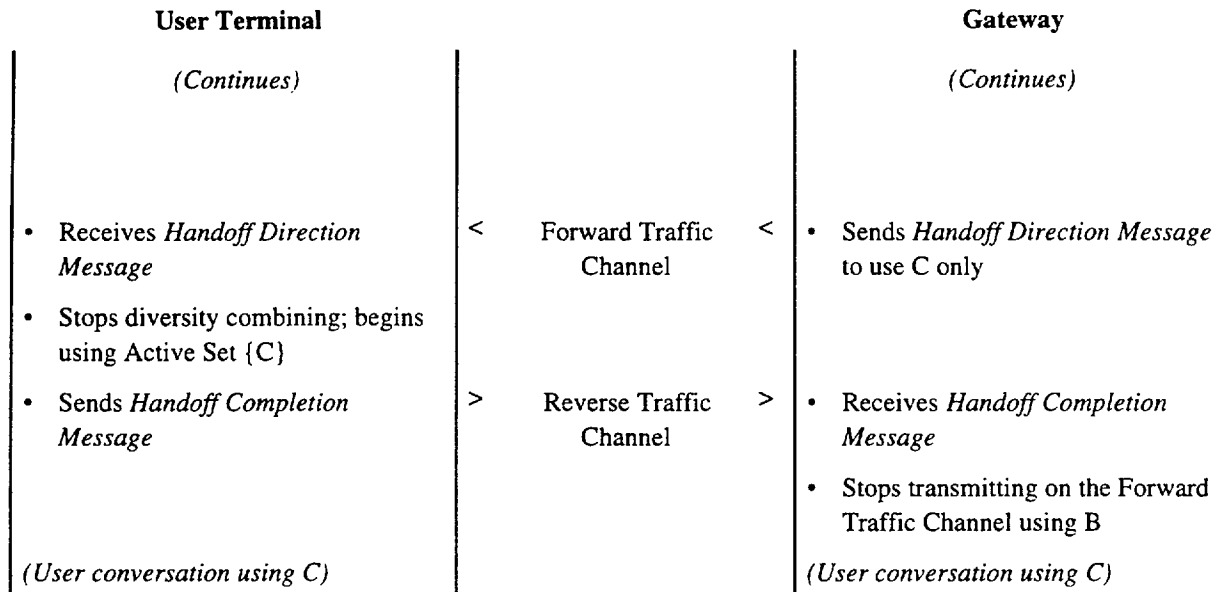
3 Figure 6-16 Call Processing During Sequential Soft Handoff 4 (Part 2 of 2) 5 6 7 8 9
