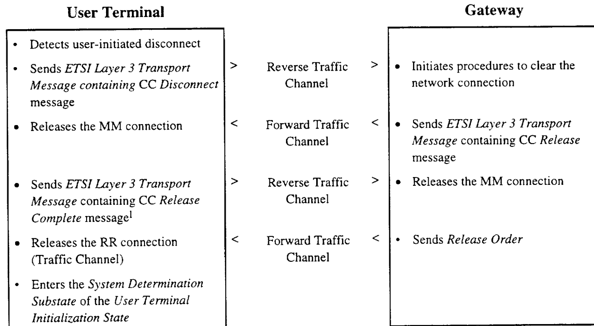
8 Figure 6-9 Simple Call Flow, User Terminal Initiated Call Disconnect Example (ETSI Call 9 Control Procedure) (Part 2 of 2)
