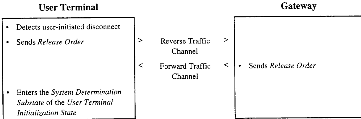
3 Figure 6-8. Simple Call Flow, User Terminal Initiated Call Disconnect Example (TIA Call 4 Control Procedures) 5 (Part 1 of 2)
