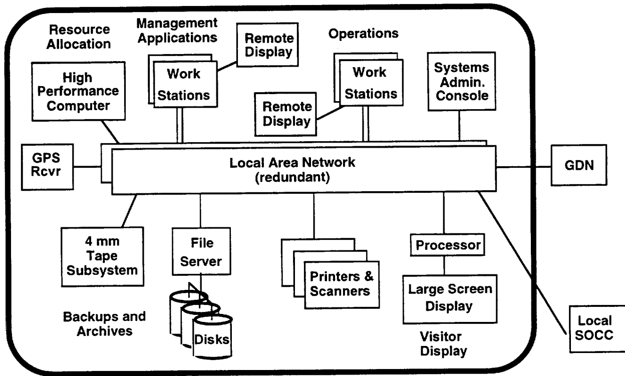
Figure 2-10 GOCC Simplified Block Diagram
