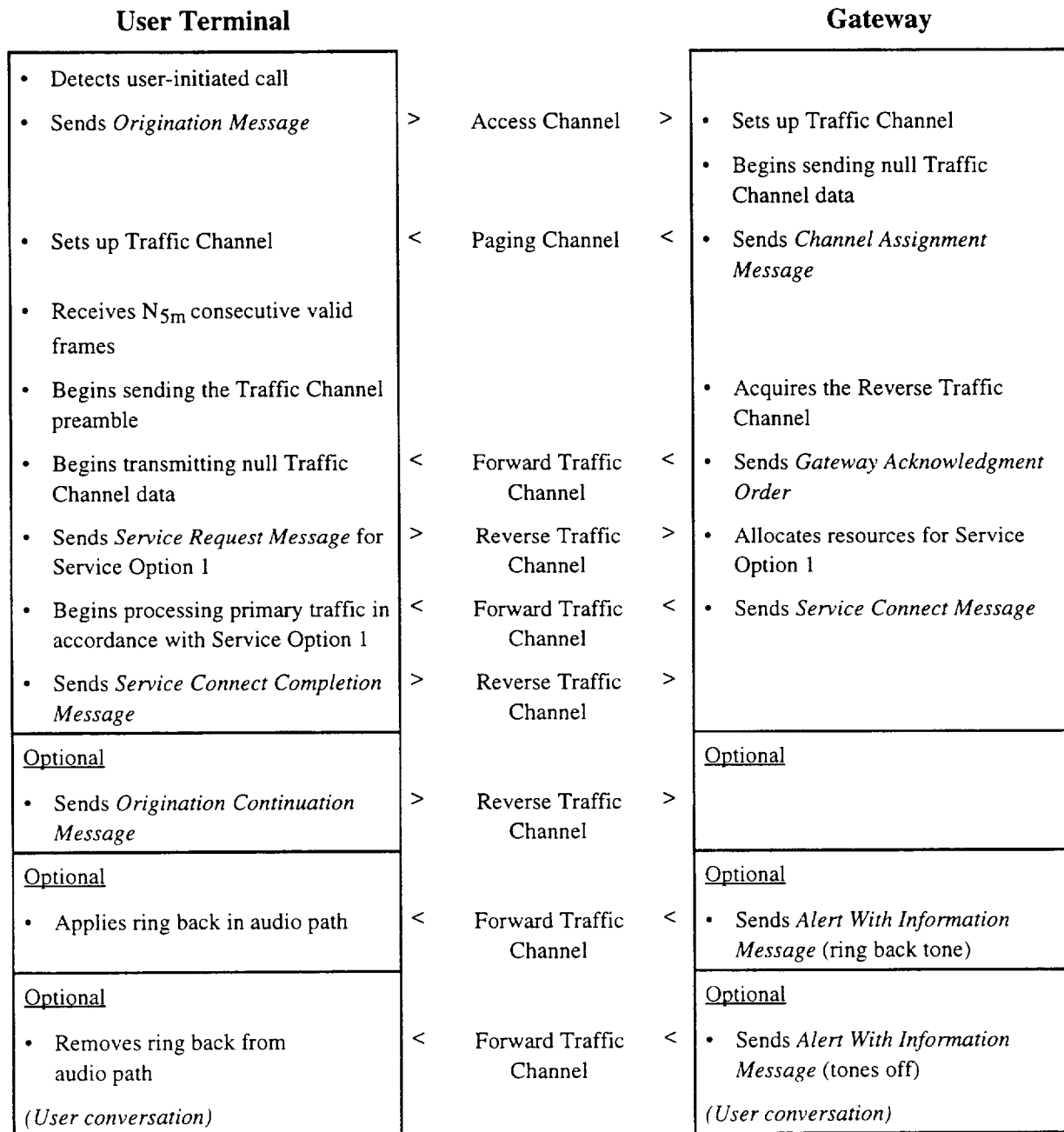
Figure 6-4 Simple Call Flow, User Terminal Origination Example Using Service Option 1 (TIA Call Control Procedures)
