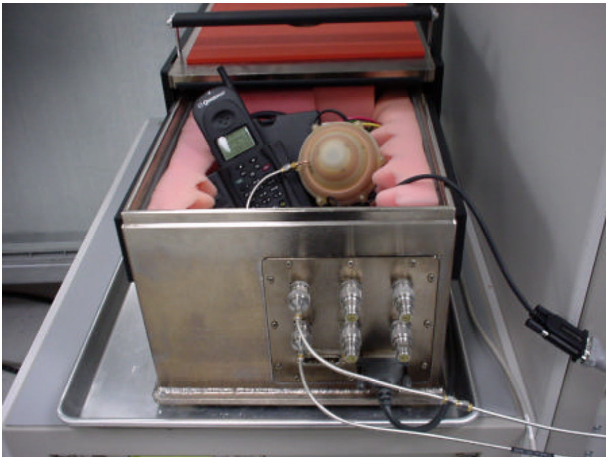
Photo C-3 GCK 1410 Car Kit in EMI enclosure for Conducted Tests
