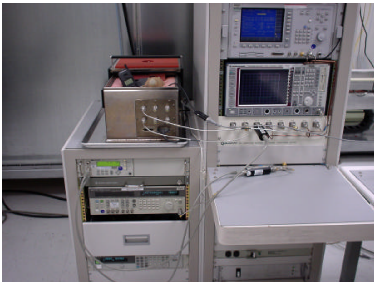
Photo C-5 GCK 1410 Car Kit shown in Conducted Test Arrangement
