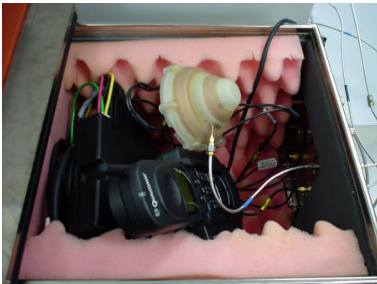
Photo C-6 GCK 1410 Car Kit in EMI enclosure for Conducted Tests (side view)
