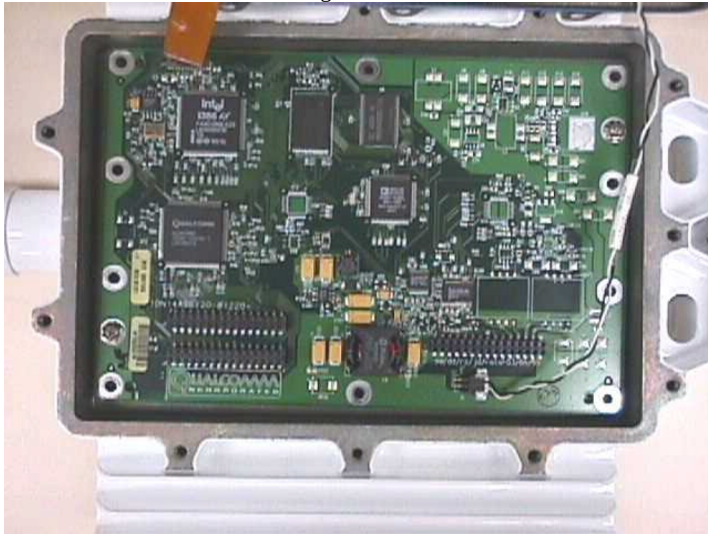
Digital Board
