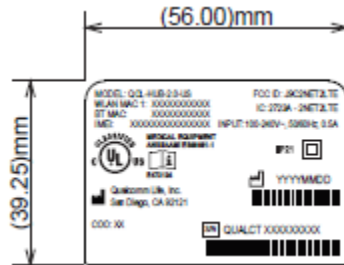
Figure 1-1 2net2 LTE Hub label shown at 100%
