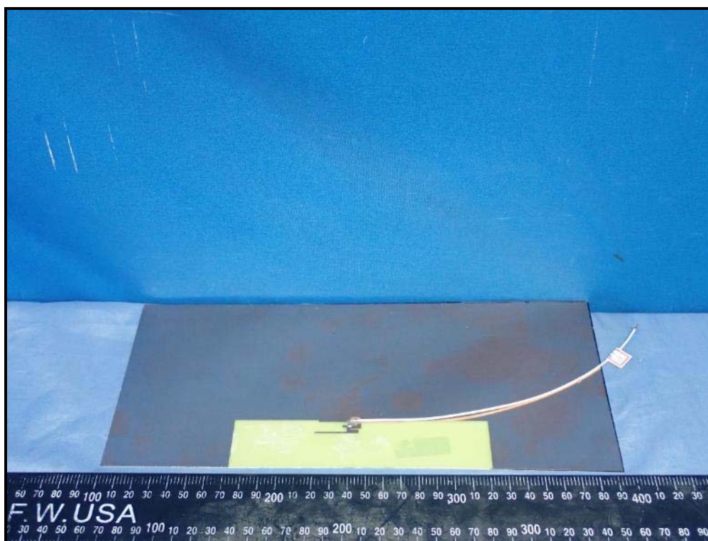
Antenna 3 (Model: 260-25084)
