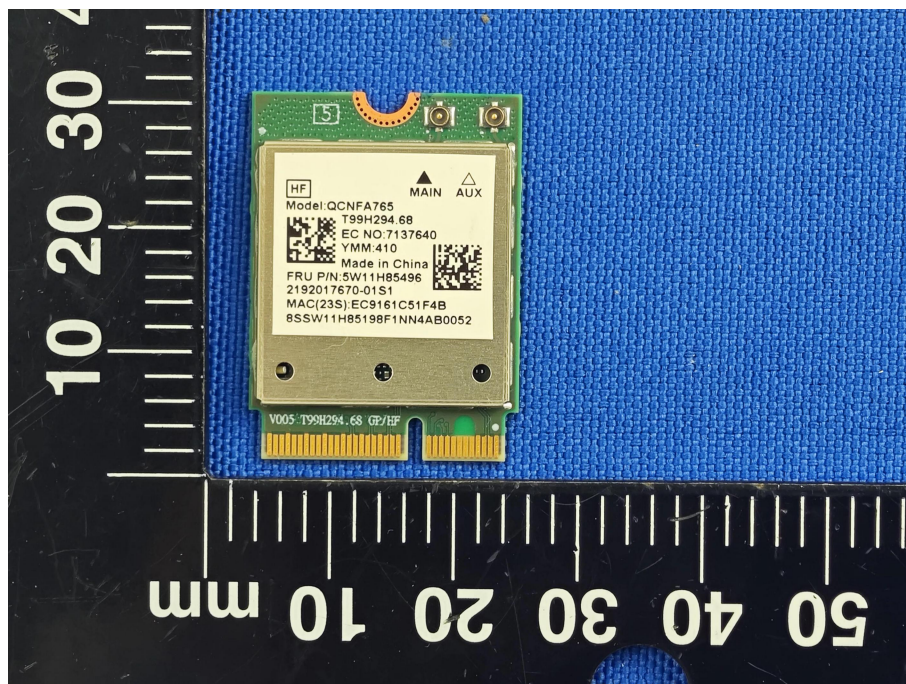
RF MODULE TOP VIEW - QCNFA765 (WITH SHIELDING)
