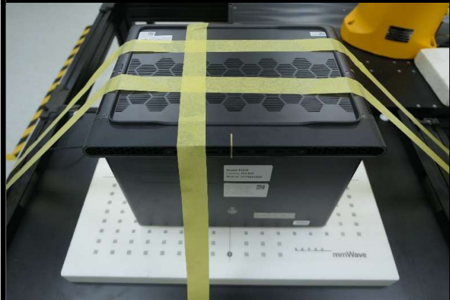
Bottom for Laptop of EUT Tested at 0 mm
