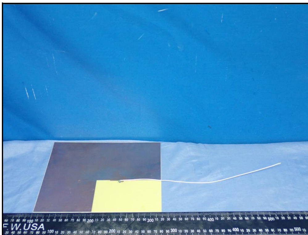
Antenna 2 (Model: 260-25083)
