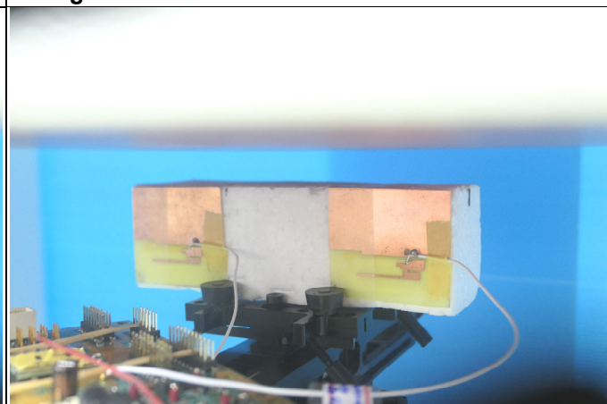
Bottom Side of EUT with SKU C Tested at 15 mm
