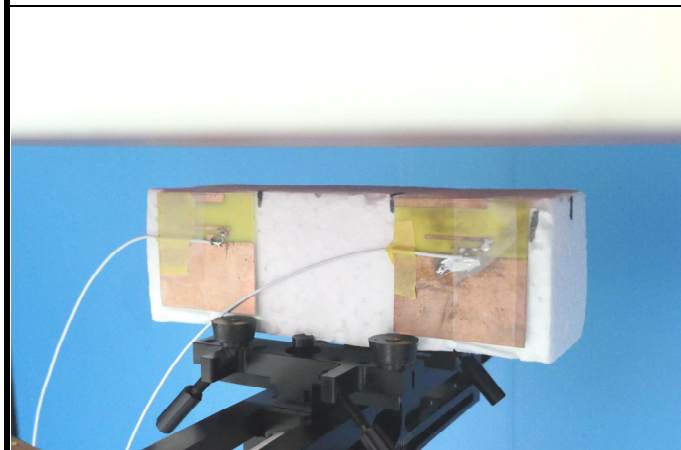
Top Side of EUT with SKU A Tested at 15 mm
