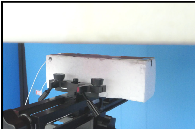
Front Face of EUT with SKU A Tested at 15 mm
