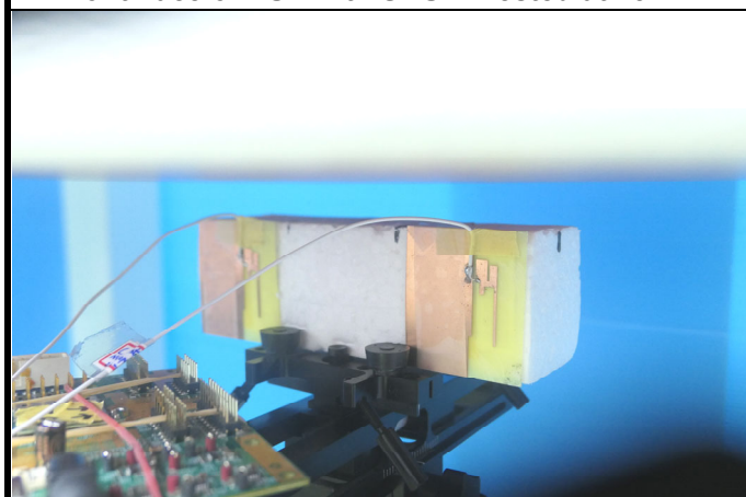
Left Side of EUT with SKU C Tested at 15 mm
