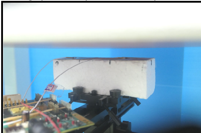
Front Face of EUT with SKU C Tested at 15 mm
