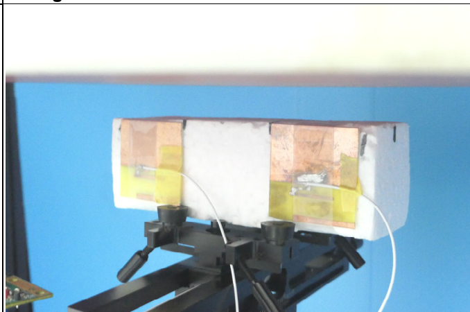
Bottom Side of EUT with SKU A Tested at 15 mm
