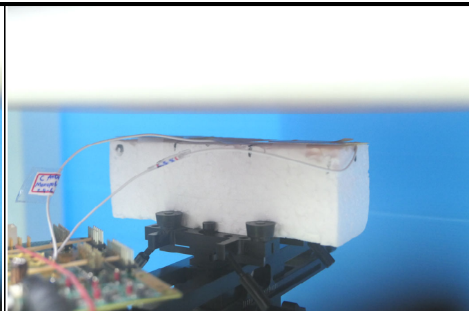
Rear Face of EUT with SKU C Tested at 15 mm
