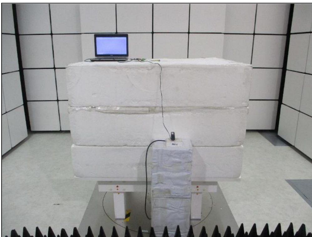
EUT with 50 ohm terminator
