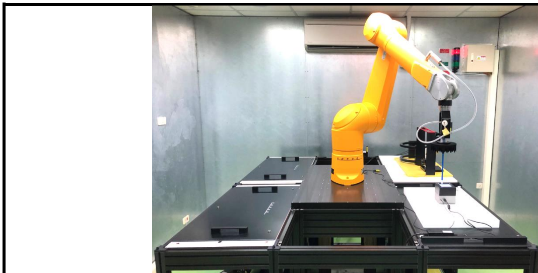
Fig-5.2 SPEAG DASY6 System
