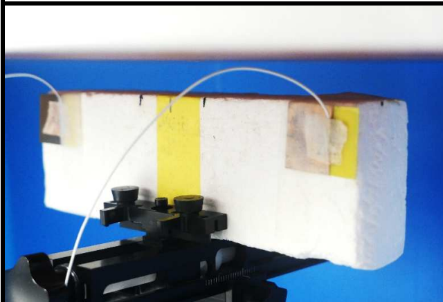
Left Side of EUT Tested at 22 mm
