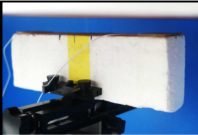
Rear Face of EUT Tested at 22 mm
