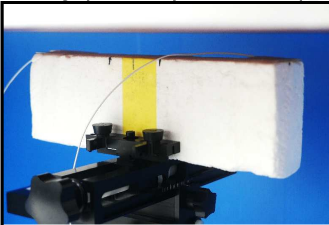
Front Face of EUT Tested at 22 mm
