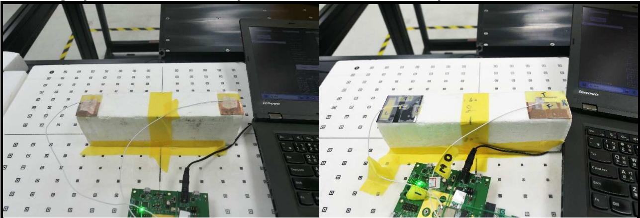
Front Face of EUT Tested at PIFA
