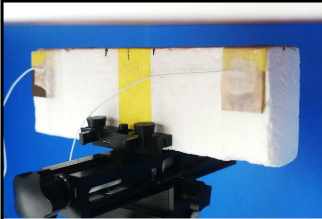
Top Side of EUT Tested at 22 mm
