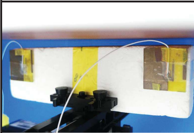
Left Side of EUT Tested at 8 mm
