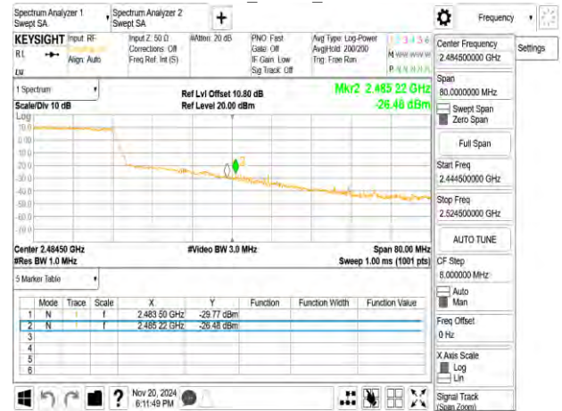
802.11ax_40MHz_2442MHz_RU242_62
