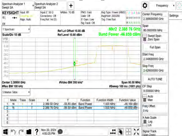
802.11ax_20MHz_2412MHz_RU106_53
