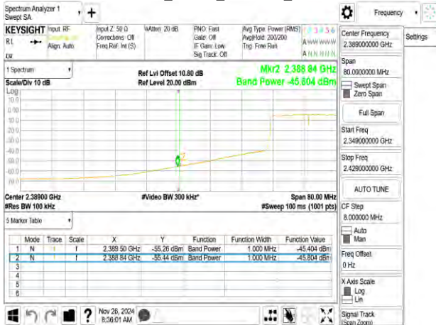
802.11ax_20MHz_2422MHz_RU26_0
