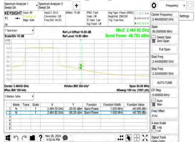
802.11ax_20MHz_2462MHz_RU106_54
