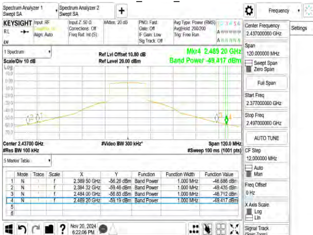
802.11ax_20MHz_2437MHz_RU106_53
