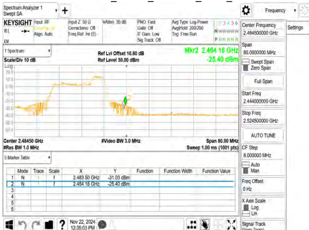
802.11ax_20MHz_2467MHz_RU52_40
