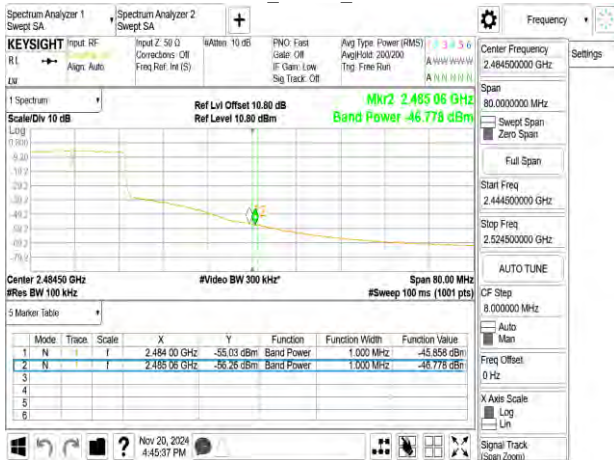
802.11ax_20MHz_2452MHz_RU106_54
