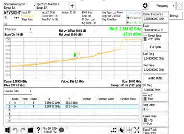
802.11ax_20MHz_2427MHz_RU106_53
