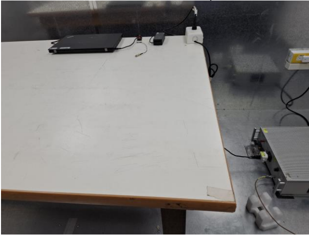
Thread_Conduction_Setup
