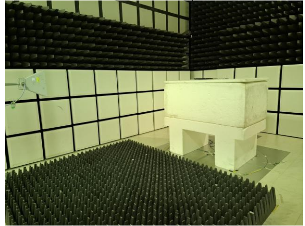
LE_Radiated_Setup
