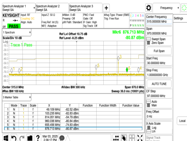
BLE_1M_Chain0_2442MHz_30M-1GHz
