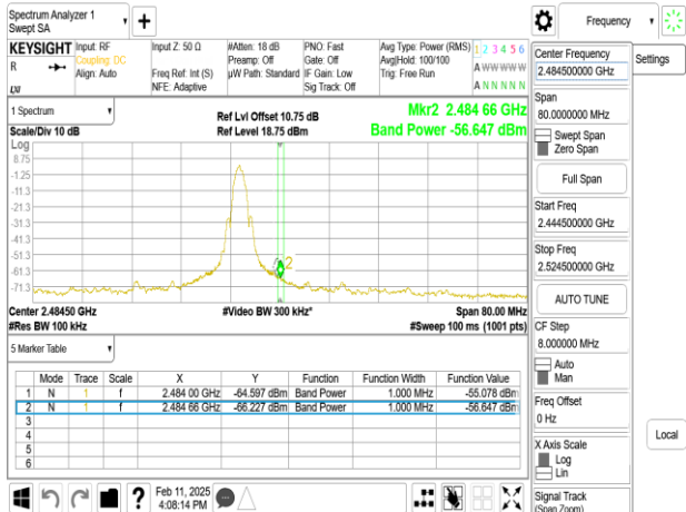
BLE_2M_Chain0_2480MHz
