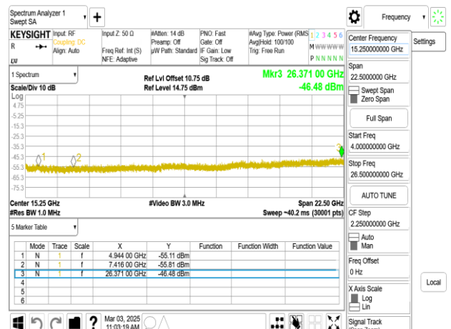
BLE_500K_Chain0_2480MHz_4-26.5GHz
