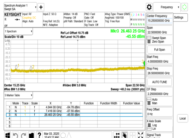
BLE_125K_Chain0_2480MHz_4-26.5GHz
