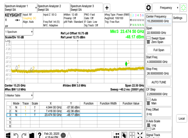
BLE_2M_Chain0_2480MHz_4-26.5GHz
