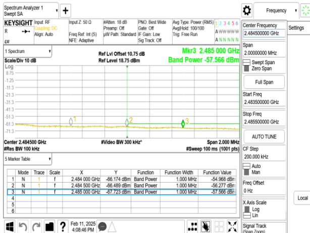
BLE_2M_Chain0_2480MHz
