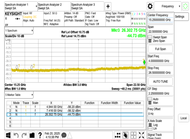
BLE_1M_Chain0_2480MHz_4-26.5GHz
