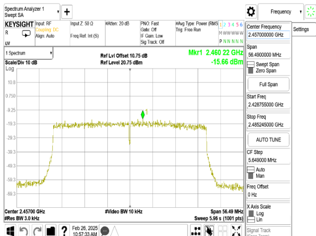
802.11ax_40MHz_Chain0_2457MHz_RU242_62
