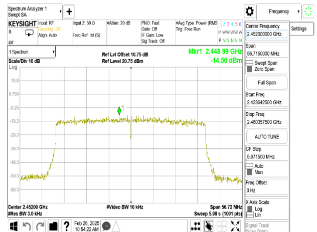
802.11ax_40MHz_Chain0_2452MHz_RU242_62
