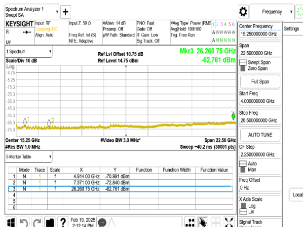
802.11ax_40MHz_Chain0_2457MHz_4-26.5GHz
