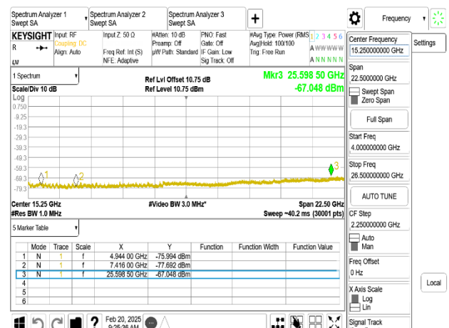
802.11ax_20MHz_Chain0_2472MHz_RU_52_40_4-26.5GHz
