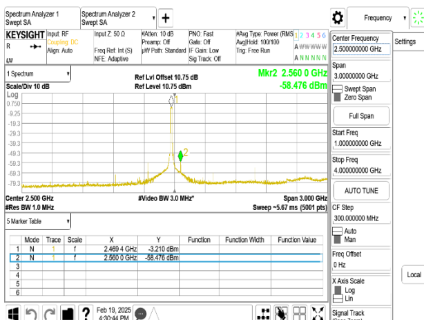
802.11ax_20MHz_Chain0_2467MHz_RU242_1-4GHz
