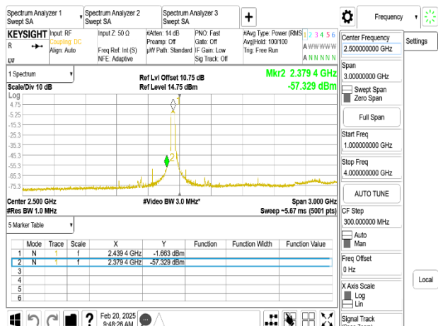
802.11ax_40MHz_Chain0_2437MHz_RU484_1-4GHz
