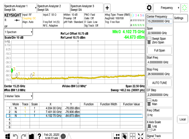
802.11ax_20MHz_Chain0_2467MHz_RU26_8_4-26.5GHz
