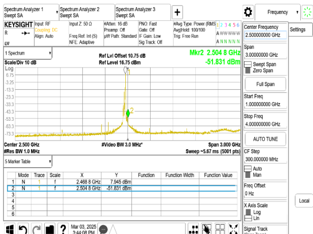
802.11ax_20MHz_Chain0_2462MHz_RU_52_40_1-4GHz
