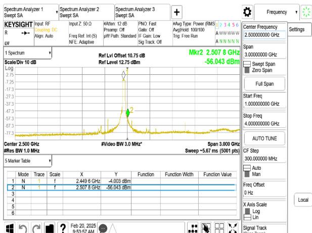
802.11ax_40MHz_Chain0_2452MHz_RU484_1-4GHz
