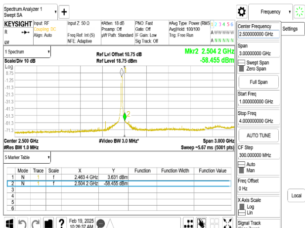
802.11g_20MHz_Chain0_2462MHz_1-4GHz
