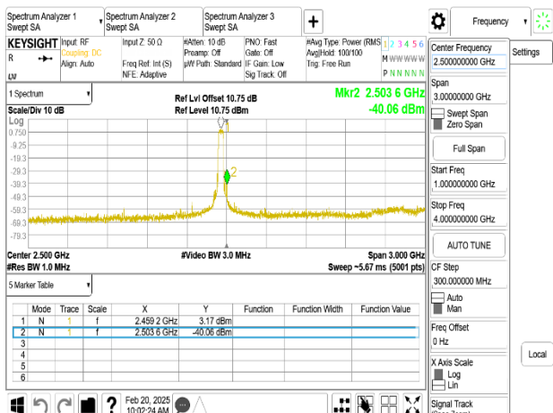
802.11ax_40MHz_Chain0_2457MHz_RU484_1-4GHz
