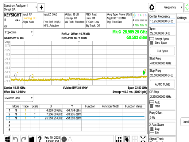
802.11ax_20MHz_Chain0_2412MHz_4-26.5GHz
