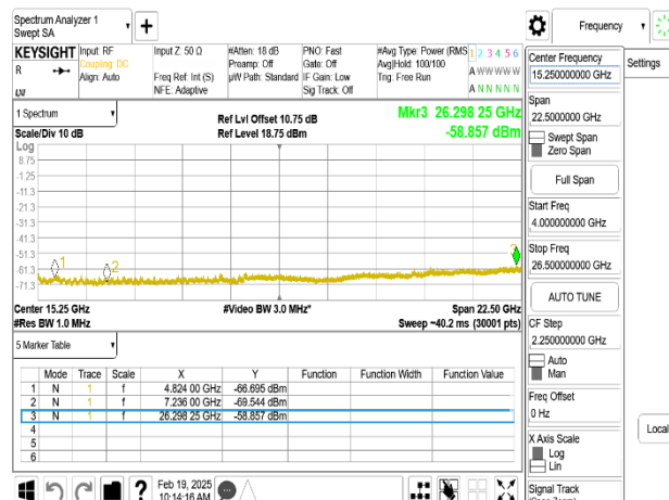
802.11g_20MHz_Chain0_2412MHz_4-26.5GHz
