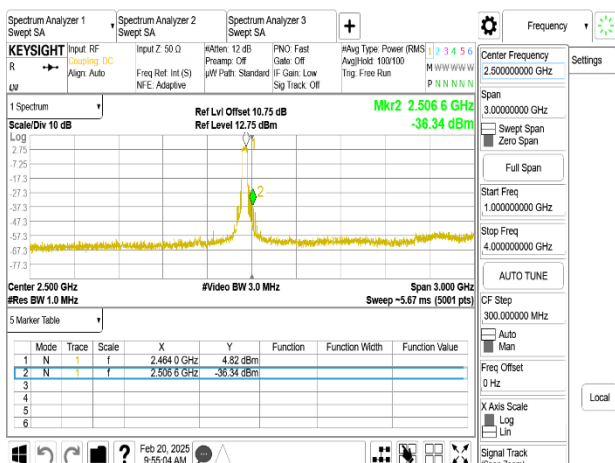
802.11ax_40MHz_Chain0_2452MHz_RU484_1-4GHz
